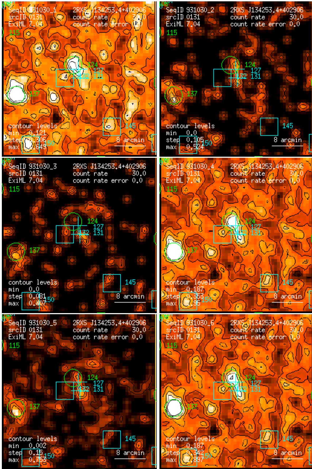
Figure 131: RASS 931030: detection 0131: band rate images, Gaussian filter: (1) PSPC channels 11 – 41, (2) 52 – 90, (3) 91 – 201, (4) 11 – 235, (5) 52 – 201, (6) 11 – 201. Broad band rates in counts/ks. Band rate contour levels in counts/ks/arcmin 2 .
