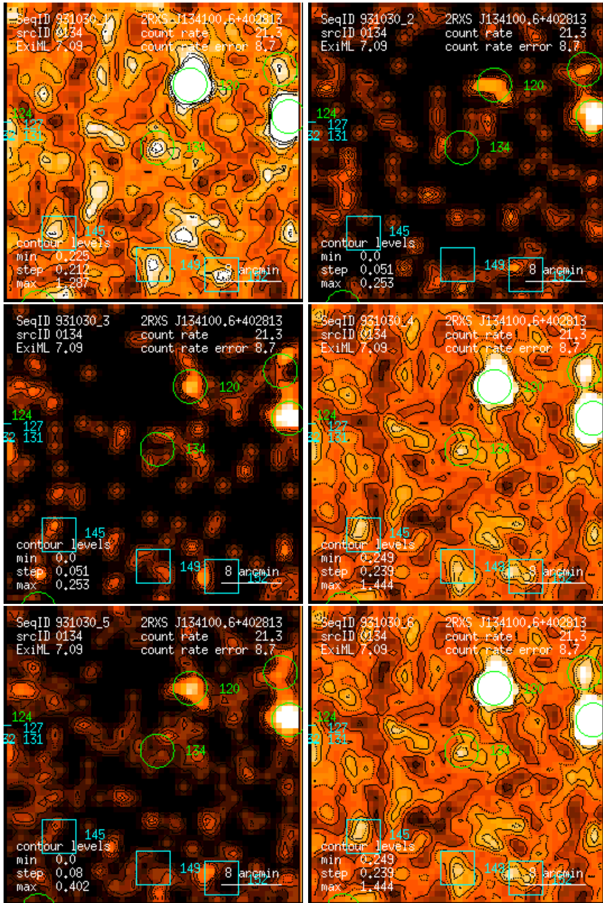
Figure 134: RASS 931030: detection 0134: band rate images, Gaussian filter: (1) PSPC channels 11 – 41, (2) 52 – 90, (3) 91 – 201, (4) 11 – 235, (5) 52 – 201, (6) 11 – 201. Broad band rates in counts/ks. Band rate contour levels in counts/ks/arcmin 2 .
