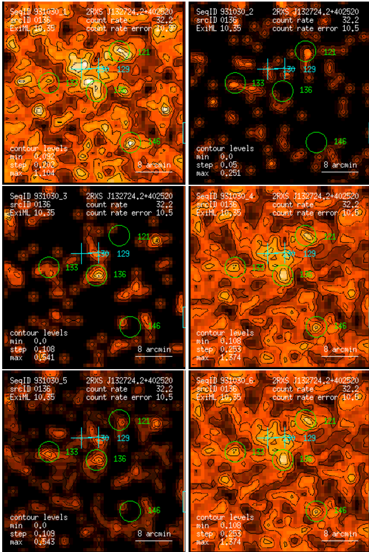
Figure 136: RASS 931030: detection 0136: band rate images, Gaussian filter: (1) PSPC channels 11 – 41, (2) 52 – 90, (3) 91 – 201, (4) 11 – 235, (5) 52 – 201, (6) 11 – 201. Broad band rates in counts/ks. Band rate contour levels in counts/ks/arcmin 2 .
