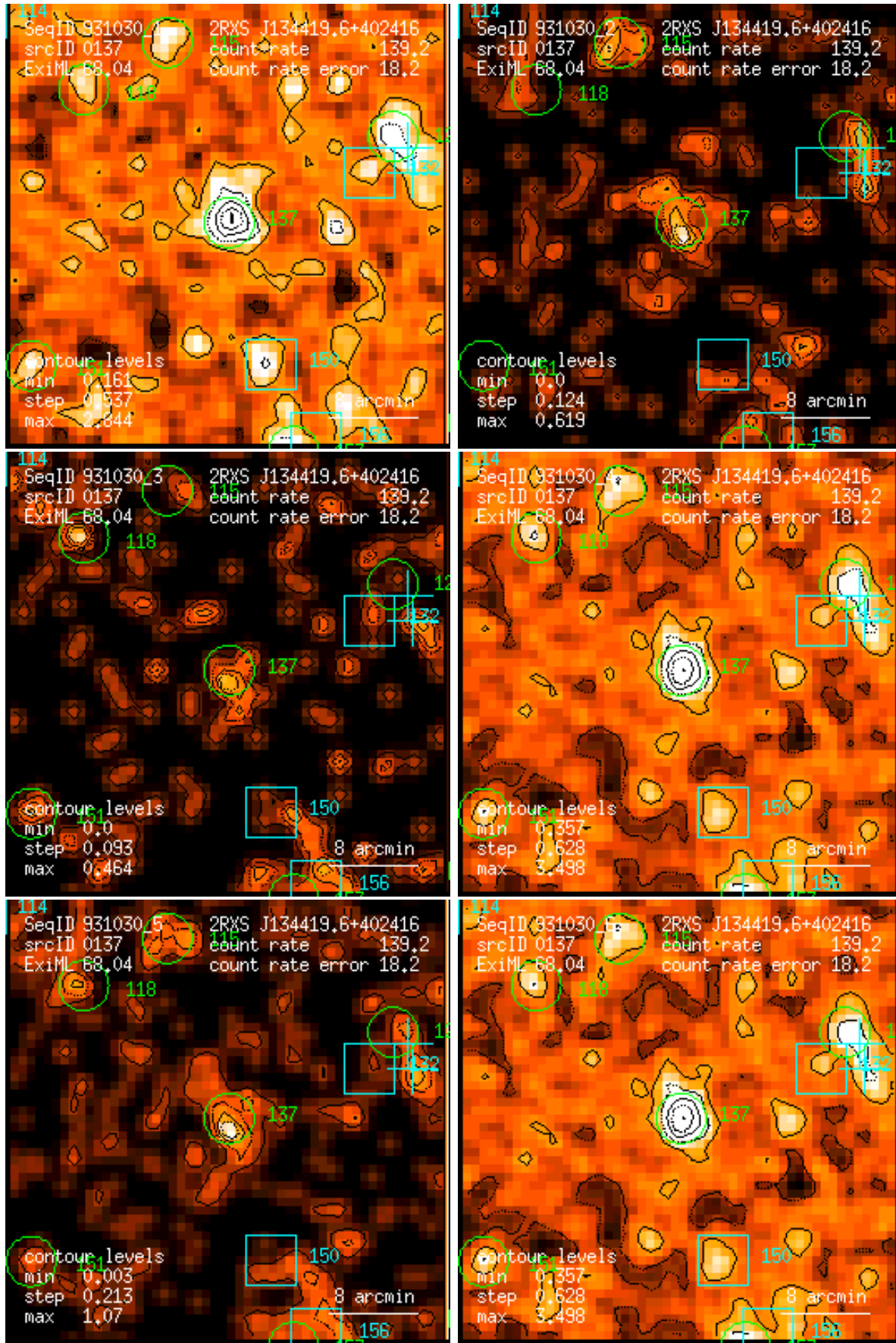
Figure 137: RASS 931030: detection 0137: band rate images, Gaussian filter: (1) PSPC channels 11 – 41, (2) 52 – 90, (3) 91 – 201, (4) 11 – 235, (5) 52 – 201, (6) 11 – 201. Broad band rates in counts/ks. Band rate contour levels in counts/ks/arcmin 2 .
