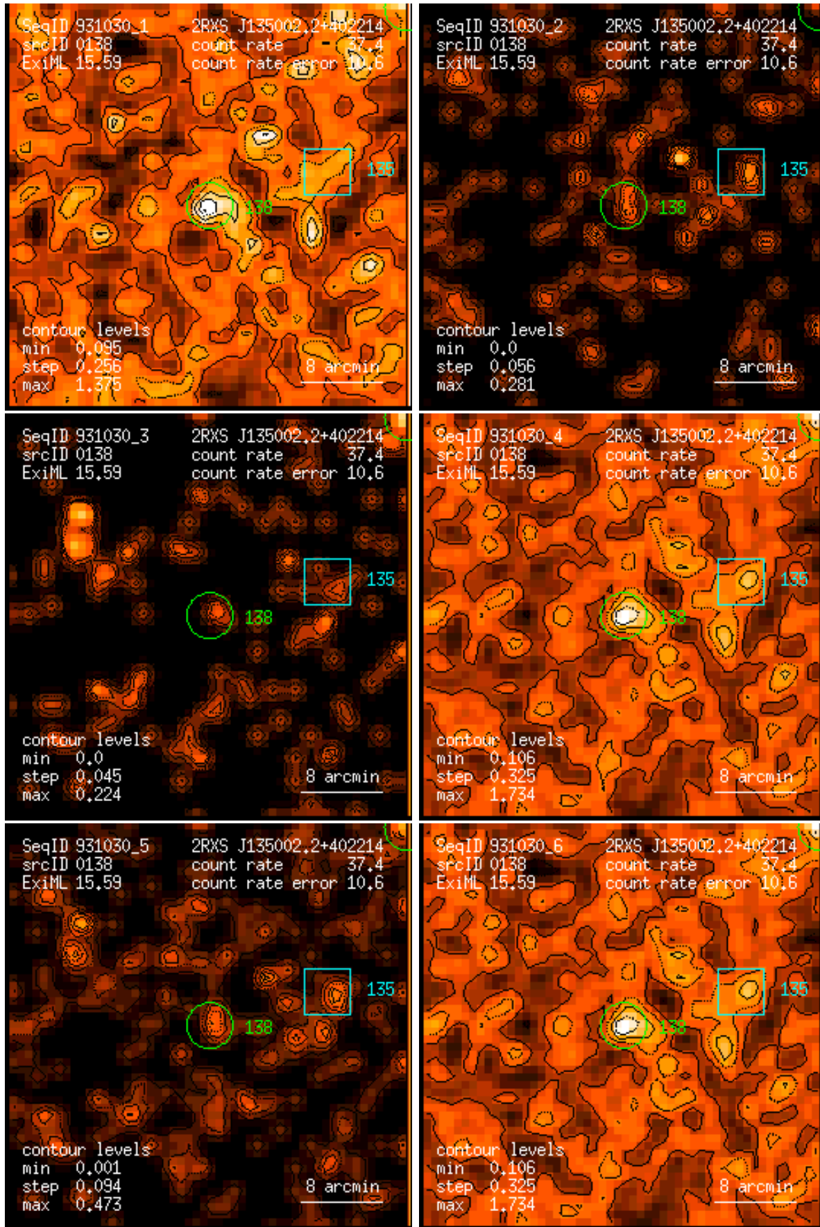
Figure 138: RASS 931030: detection 0138: band rate images, Gaussian filter: (1) PSPC channels 11 – 41, (2) 52 – 90, (3) 91 – 201, (4) 11 – 235, (5) 52 – 201, (6) 11 – 201. Broad band rates in counts/ks. Band rate contour levels in counts/ks/arcmin 2 .
