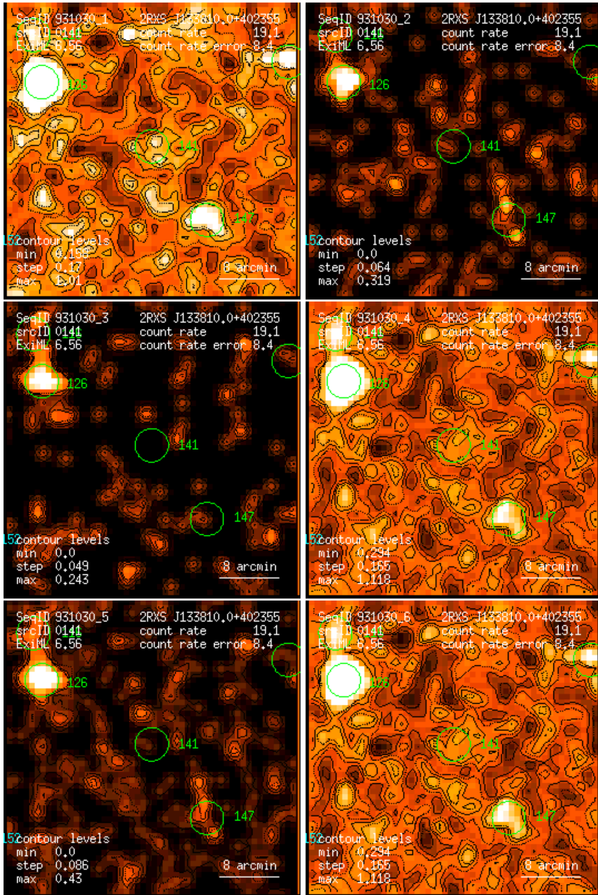
Figure 141: RASS 931030: detection 0141: band rate images, Gaussian filter: (1) PSPC channels 11 – 41, (2) 52 – 90, (3) 91 – 201, (4) 11 – 235, (5) 52 – 201, (6) 11 – 201. Broad band rates in counts/ks. Band rate contour levels in counts/ks/arcmin 2 .
