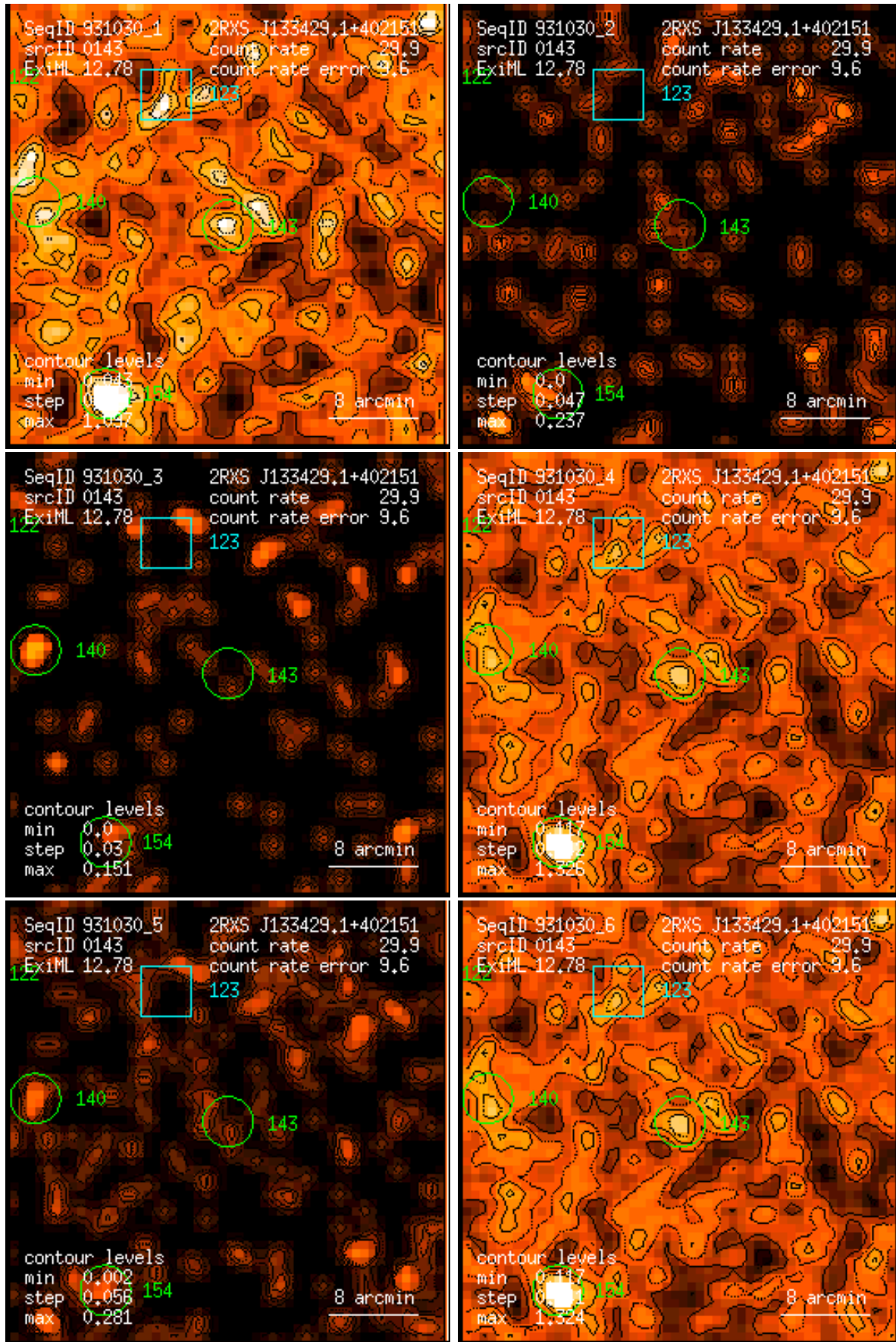
Figure 143: RASS 931030: detection 0143: band rate images, Gaussian filter: (1) PSPC channels 11 – 41, (2) 52 – 90, (3) 91 – 201, (4) 11 – 235, (5) 52 – 201, (6) 11 – 201. Broad band rates in counts/ks. Band rate contour levels in counts/ks/arcmin 2 .
