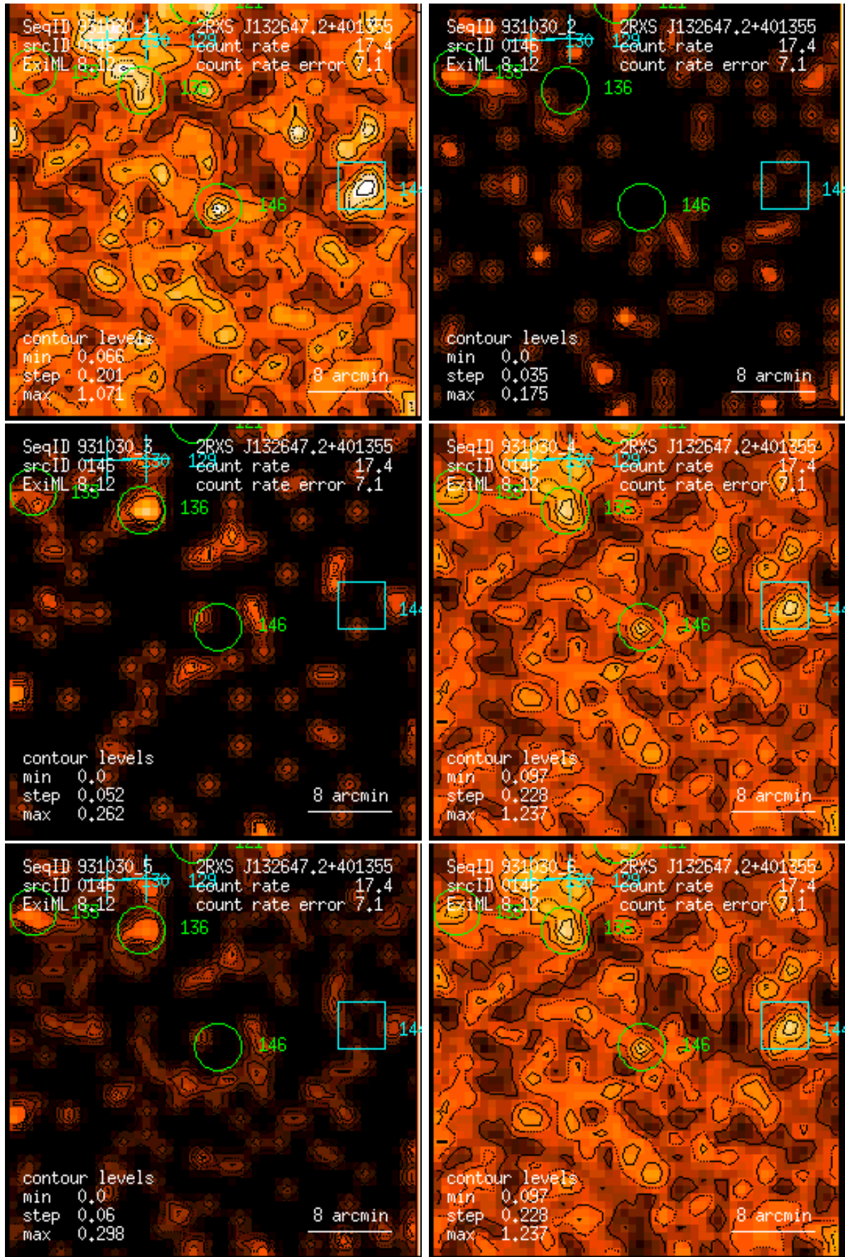
Figure 146: RASS 931030: detection 0146: band rate images, Gaussian filter: (1) PSPC channels 11 – 41, (2) 52 – 90, (3) 91 – 201, (4) 11 – 235, (5) 52 – 201, (6) 11 – 201. Broad band rates in counts/ks. Band rate contour levels in counts/ks/arcmin 2 .
