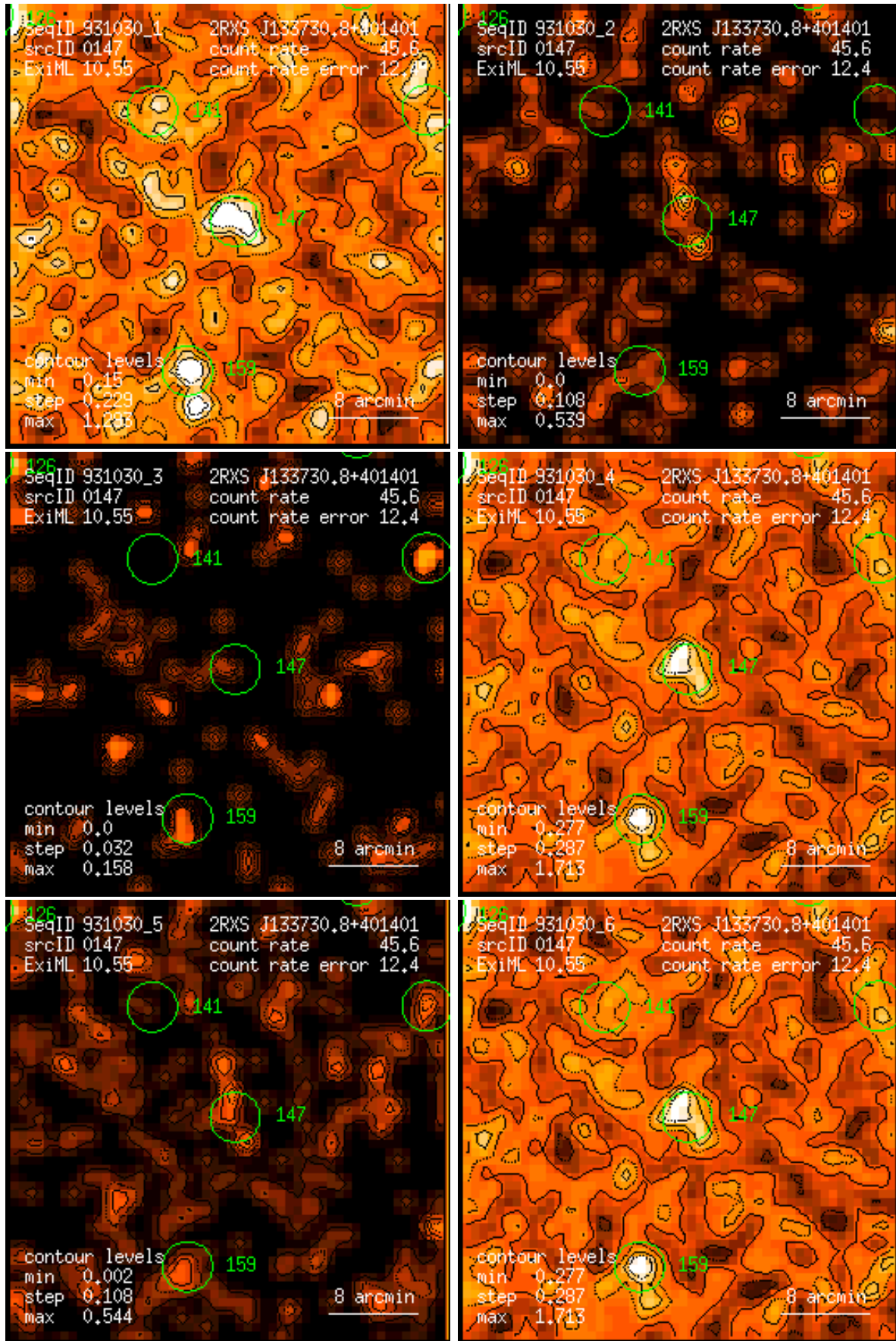
Figure 147: RASS 931030: detection 0147: band rate images, Gaussian filter: (1) PSPC channels 11 – 41, (2) 52 – 90, (3) 91 – 201, (4) 11 – 235, (5) 52 – 201, (6) 11 – 201. Broad band rates in counts/ks. Band rate contour levels in counts/ks/arcmin 2 .
