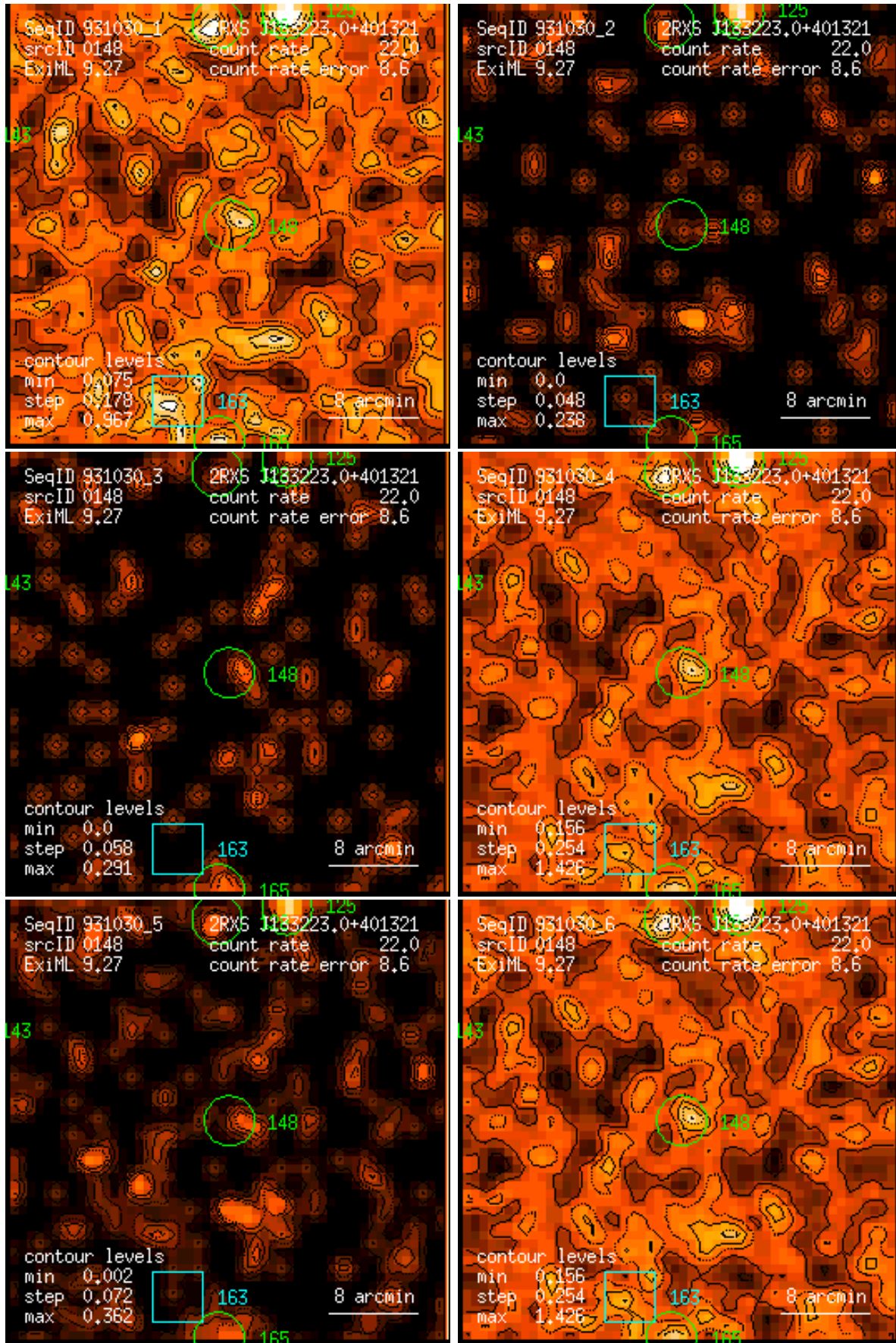
Figure 148: RASS 931030: detection 0148: band rate images, Gaussian filter: (1) PSPC channels 11 – 41, (2) 52 – 90, (3) 91 – 201, (4) 11 – 235, (5) 52 – 201, (6) 11 – 201. Broad band rates in counts/ks. Band rate contour levels in counts/ks/arcmin 2 .
