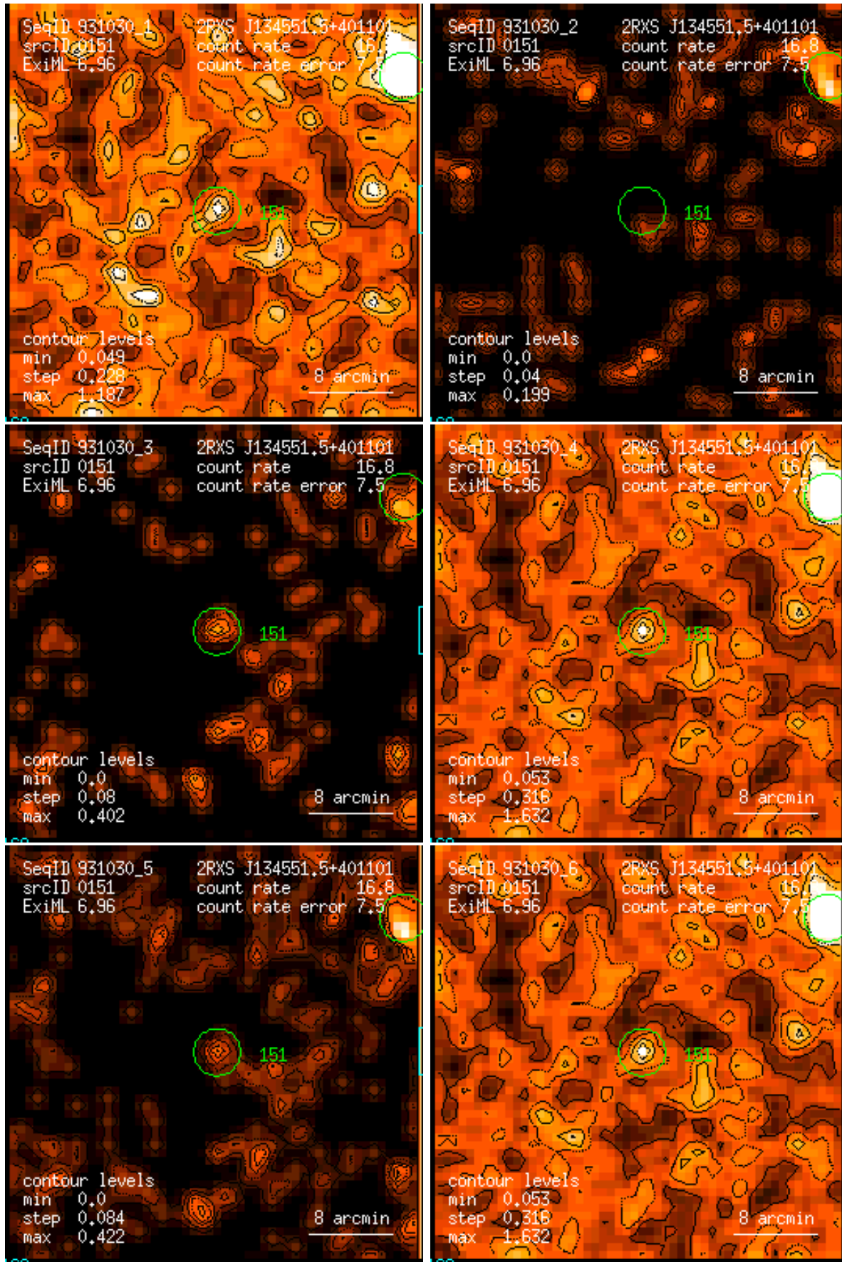
Figure 151: RASS 931030: detection 0151: band rate images, Gaussian filter: (1) PSPC channels 11 – 41, (2) 52 – 90, (3) 91 – 201, (4) 11 – 235, (5) 52 – 201, (6) 11 – 201. Broad band rates in counts/ks. Band rate contour levels in counts/ks/arcmin 2 .
