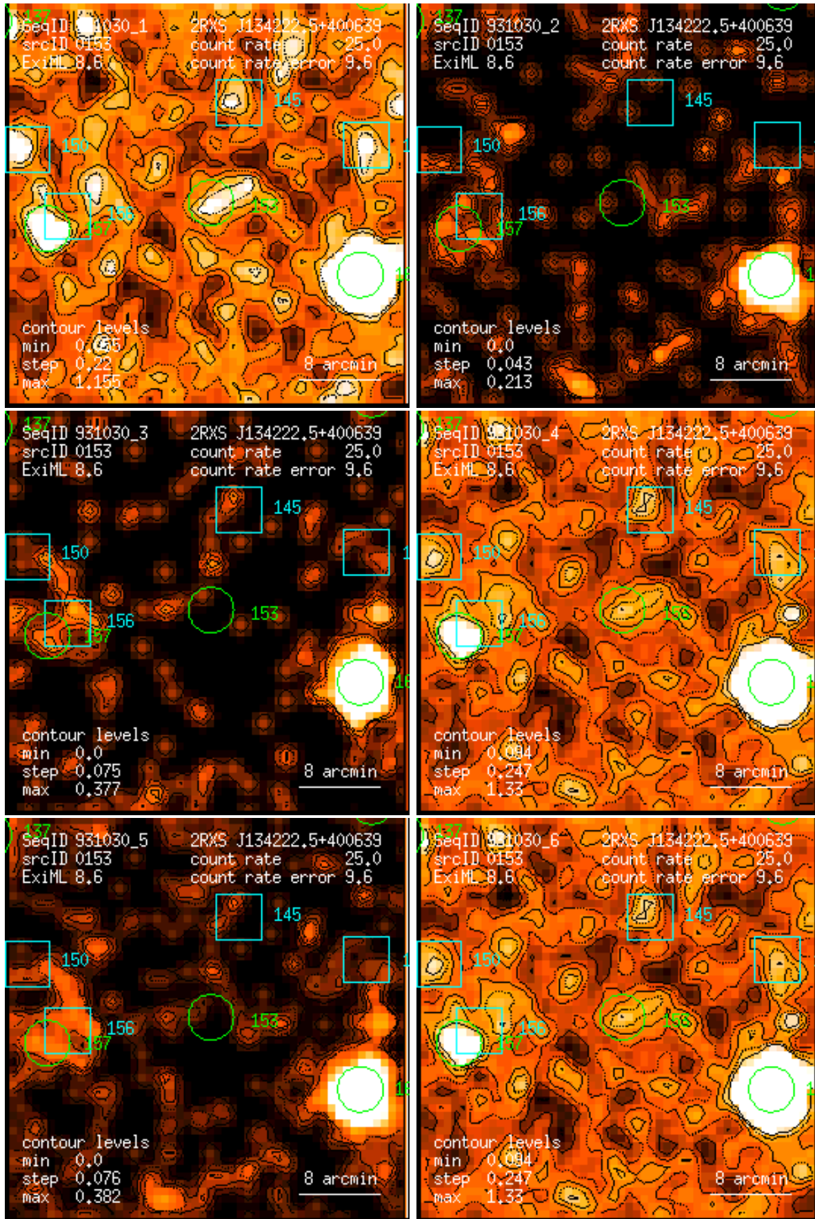
Figure 153: RASS 931030: detection 0153: band rate images, Gaussian filter: (1) PSPC channels 11 – 41, (2) 52 – 90, (3) 91 – 201, (4) 11 – 235, (5) 52 – 201, (6) 11 – 201. Broad band rates in counts/ks. Band rate contour levels in counts/ks/arcmin 2 .
