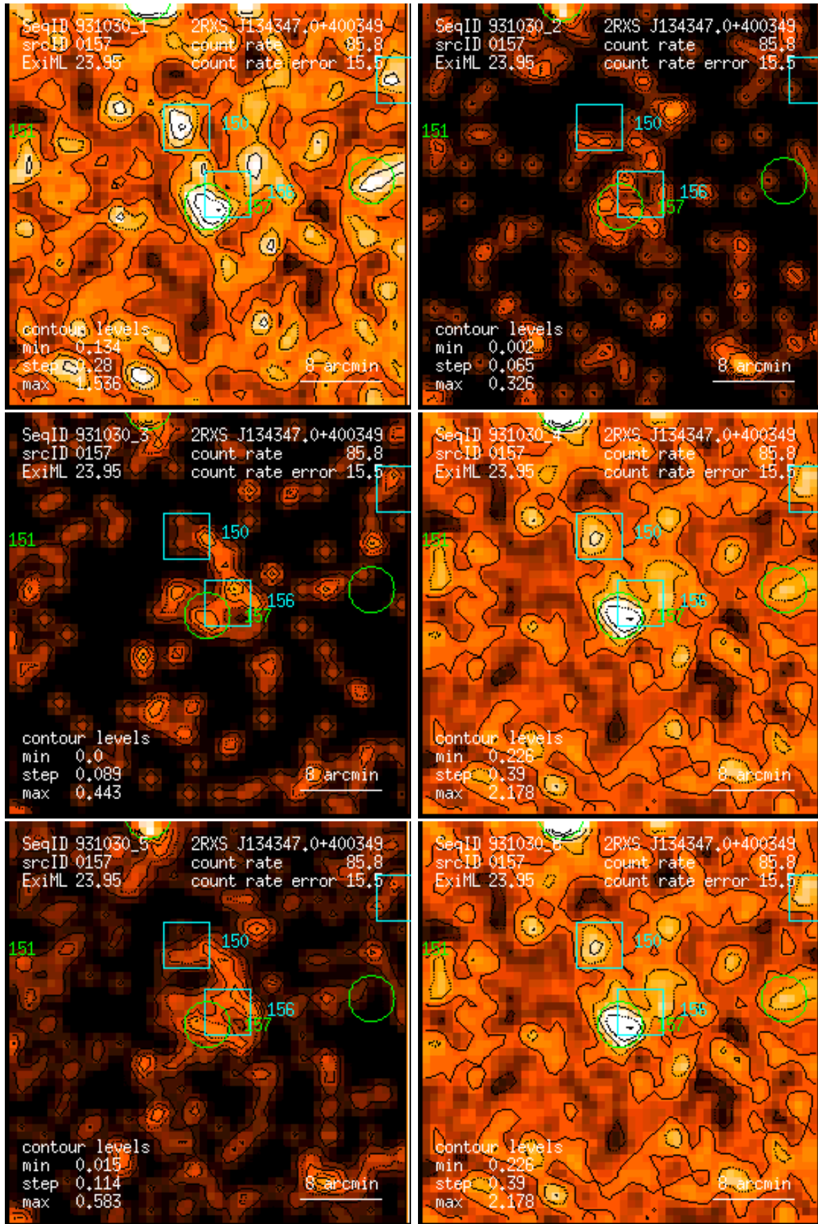
Figure 157: RASS 931030: detection 0157: band rate images, Gaussian filter: (1) PSPC channels 11 – 41, (2) 52 – 90, (3) 91 – 201, (4) 11 – 235, (5) 52 – 201, (6) 11 – 201. Broad band rates in counts/ks. Band rate contour levels in counts/ks/arcmin 2 .
