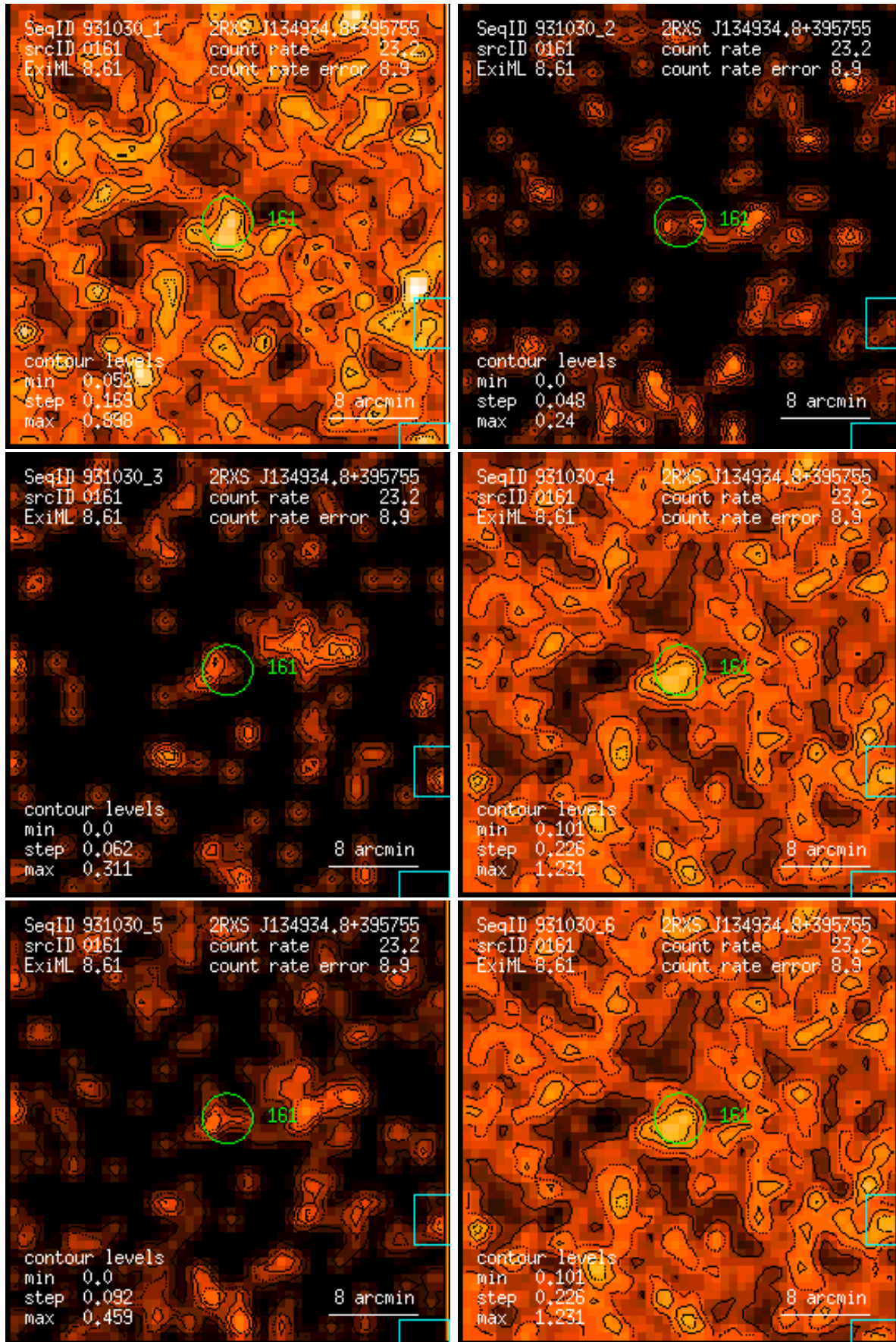
Figure 161: RASS 931030: detection 0161: band rate images, Gaussian filter: (1) PSPC channels 11 – 41, (2) 52 – 90, (3) 91 – 201, (4) 11 – 235, (5) 52 – 201, (6) 11 – 201. Broad band rates in counts/ks. Band rate contour levels in counts/ks/arcmin 2 .
