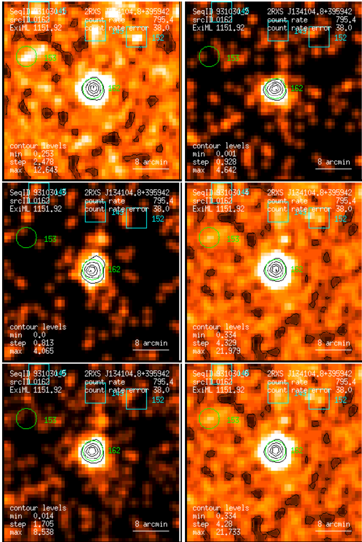
Figure 162: RASS 931030: detection 0162: band rate images, Gaussian filter: (1) PSPC channels 11 – 41, (2) 52 – 90, (3) 91 – 201, (4) 11 – 235, (5) 52 – 201, (6) 11 – 201. Broad band rates in counts/ks. Band rate contour levels in counts/ks/arcmin 2 .
