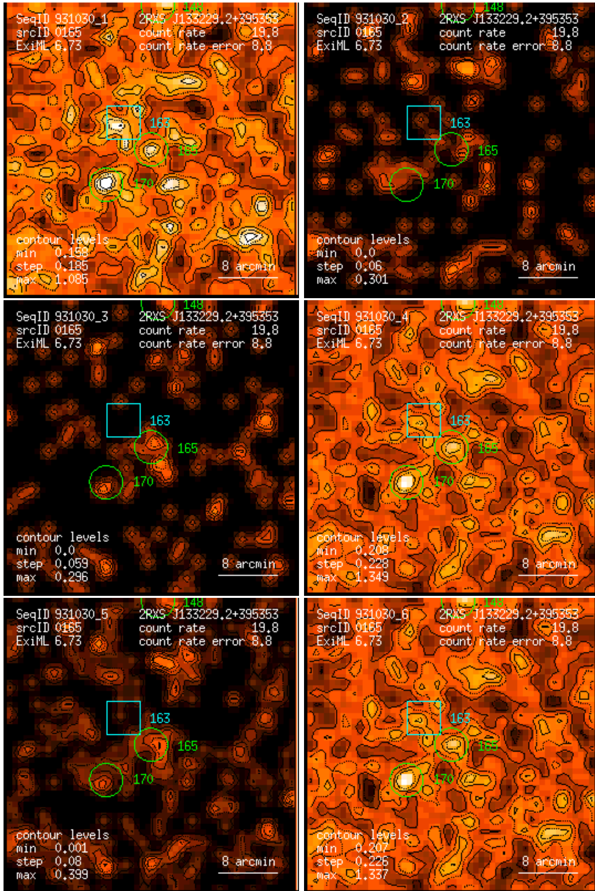
Figure 165: RASS 931030: detection 0165: band rate images, Gaussian filter: (1) PSPC channels 11 – 41, (2) 52 – 90, (3) 91 – 201, (4) 11 – 235, (5) 52 – 201, (6) 11 – 201. Broad band rates in counts/ks. Band rate contour levels in counts/ks/arcmin 2 .
