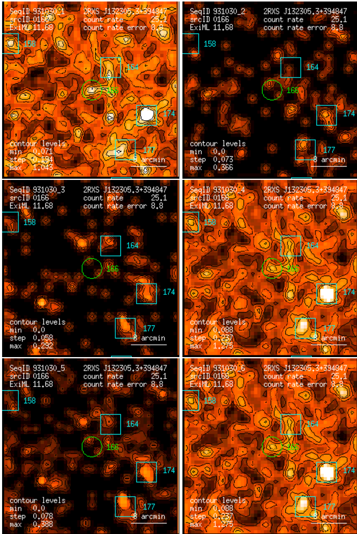
Figure 166: RASS 931030: detection 0166: band rate images, Gaussian filter: (1) PSPC channels 11 – 41, (2) 52 – 90, (3) 91 – 201, (4) 11 – 235, (5) 52 – 201, (6) 11 – 201. Broad band rates in counts/ks. Band rate contour levels in counts/ks/arcmin 2 .
