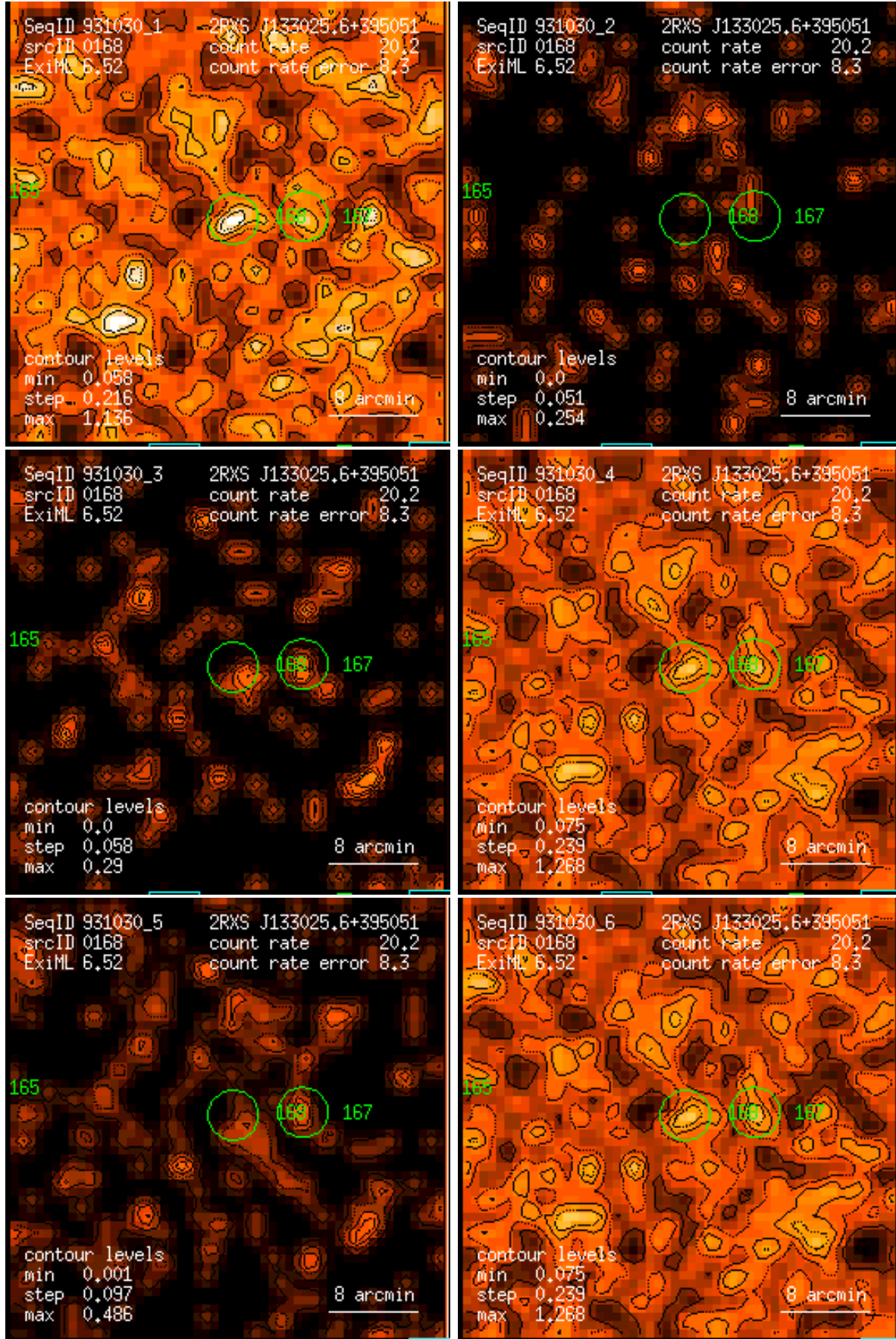
Figure 168: RASS 931030: detection 0168: band rate images, Gaussian filter: (1) PSPC channels 11 – 41, (2) 52 – 90, (3) 91 – 201, (4) 11 – 235, (5) 52 – 201, (6) 11 – 201. Broad band rates in counts/ks. Band rate contour levels in counts/ks/arcmin 2 .
