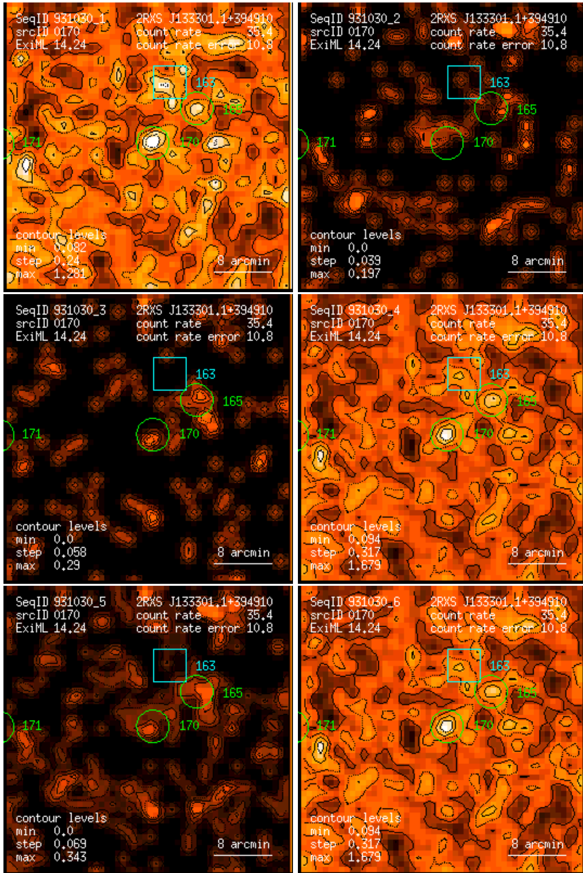
Figure 170: RASS 931030: detection 0170: band rate images, Gaussian filter: (1) PSPC channels 11 – 41, (2) 52 – 90, (3) 91 – 201, (4) 11 – 235, (5) 52 – 201, (6) 11 – 201. Broad band rates in counts/ks. Band rate contour levels in counts/ks/arcmin 2 .
