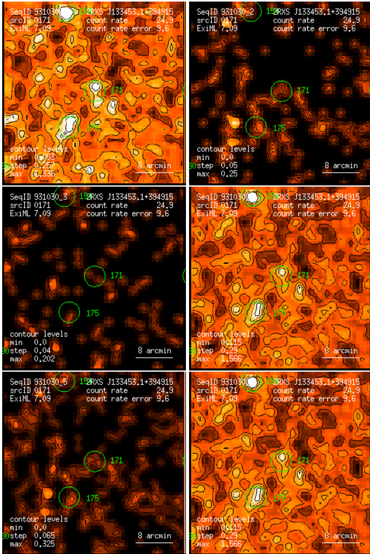
Figure 171: RASS 931030: detection 0171: band rate images, Gaussian filter: (1) PSPC channels 11 – 41, (2) 52 – 90, (3) 91 – 201, (4) 11 – 235, (5) 52 – 201, (6) 11 – 201. Broad band rates in counts/ks. Band rate contour levels in counts/ks/arcmin 2 .
