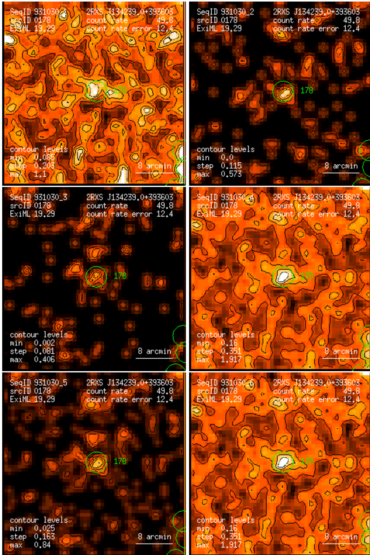
Figure 178: RASS 931030: detection 0178: band rate images, Gaussian filter: (1) PSPC channels 11 – 41, (2) 52 – 90, (3) 91 – 201, (4) 11 – 235, (5) 52 – 201, (6) 11 – 201. Broad band rates in counts/ks. Band rate contour levels in counts/ks/arcmin 2 .
