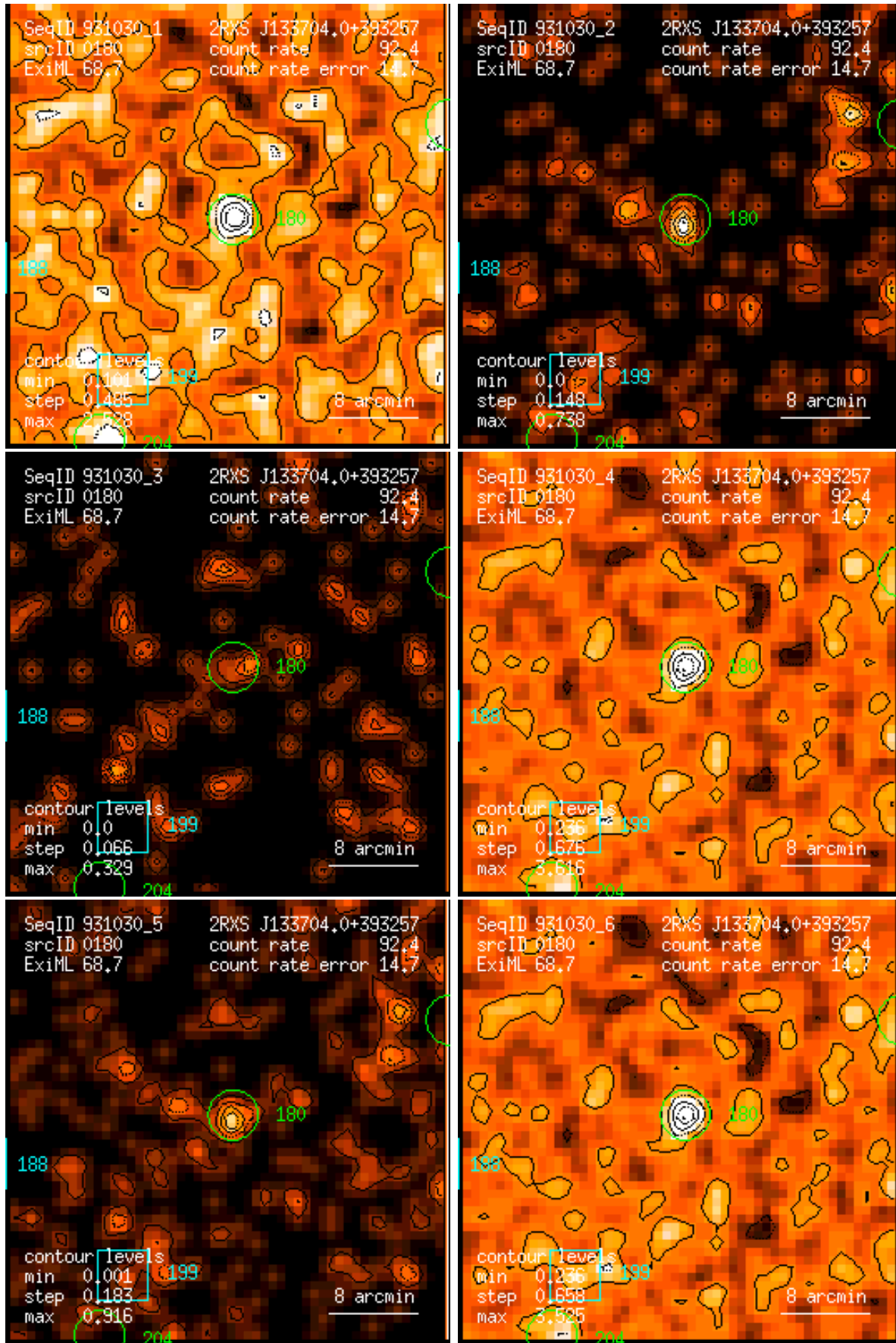
Figure 180: RASS 931030: detection 0180: band rate images, Gaussian filter: (1) PSPC channels 11 – 41, (2) 52 – 90, (3) 91 – 201, (4) 11 – 235, (5) 52 – 201, (6) 11 – 201. Broad band rates in counts/ks. Band rate contour levels in counts/ks/arcmin 2 .
