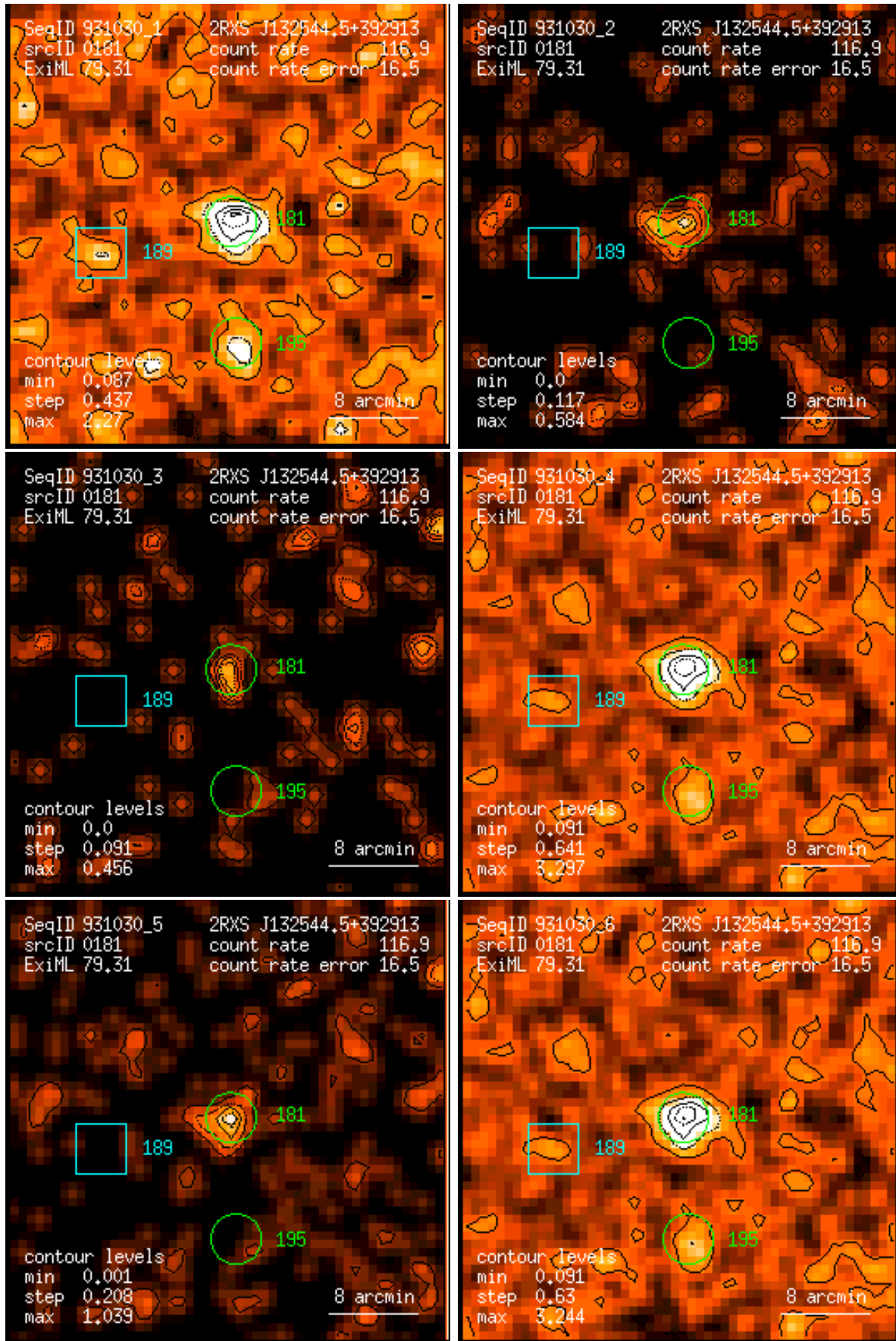
Figure 181: RASS 931030: detection 0181: band rate images, Gaussian filter: (1) PSPC channels 11 – 41, (2) 52 – 90, (3) 91 – 201, (4) 11 – 235, (5) 52 – 201, (6) 11 – 201. Broad band rates in counts/ks. Band rate contour levels in counts/ks/arcmin 2 .
