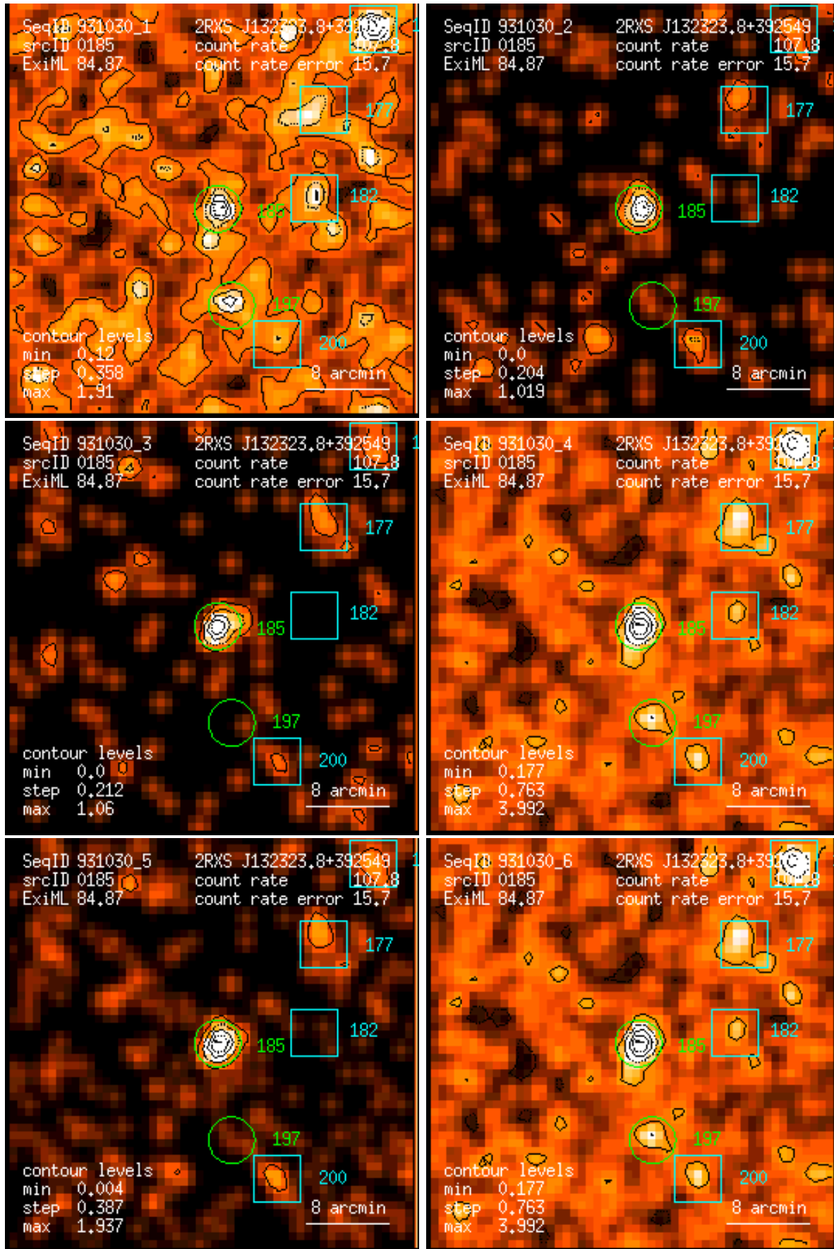
Figure 185: RASS 931030: detection 0185: band rate images, Gaussian filter: (1) PSPC channels 11 – 41, (2) 52 – 90, (3) 91 – 201, (4) 11 – 235, (5) 52 – 201, (6) 11 – 201. Broad band rates in counts/ks. Band rate contour levels in counts/ks/arcmin 2 .
