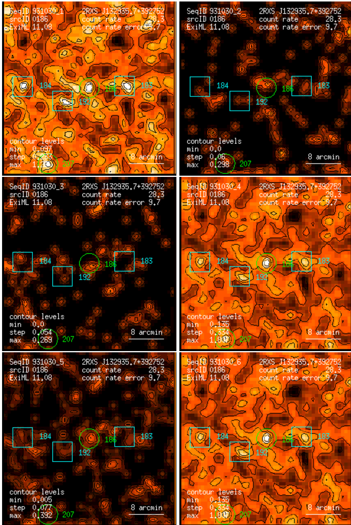
Figure 186: RASS 931030: detection 0186: band rate images, Gaussian filter: (1) PSPC channels 11 – 41, (2) 52 – 90, (3) 91 – 201, (4) 11 – 235, (5) 52 – 201, (6) 11 – 201. Broad band rates in counts/ks. Band rate contour levels in counts/ks/arcmin 2 .
