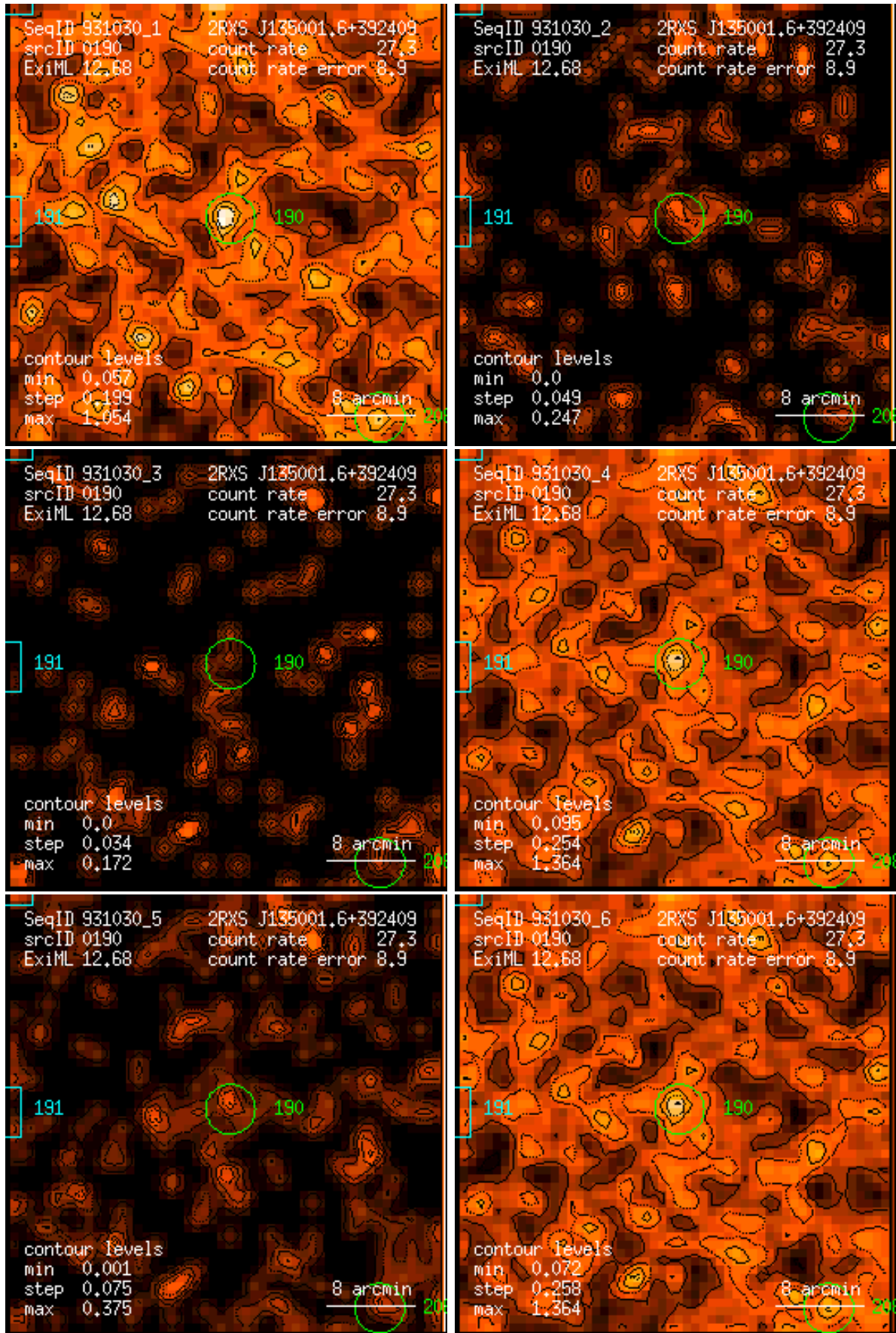
Figure 190: RASS 931030: detection 0190: band rate images, Gaussian filter: (1) PSPC channels 11 – 41, (2) 52 – 90, (3) 91 – 201, (4) 11 – 235, (5) 52 – 201, (6) 11 – 201. Broad band rates in counts/ks. Band rate contour levels in counts/ks/arcmin 2 .
