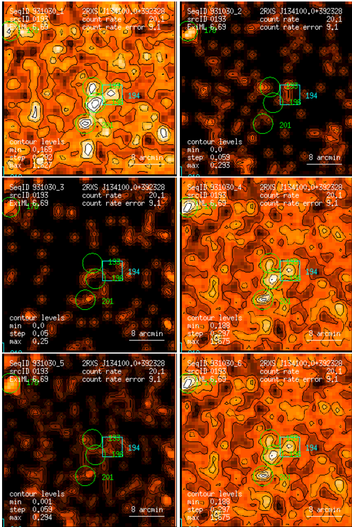
Figure 193: RASS 931030: detection 0193: band rate images, Gaussian filter: (1) PSPC channels 11 – 41, (2) 52 – 90, (3) 91 – 201, (4) 11 – 235, (5) 52 – 201, (6) 11 – 201. Broad band rates in counts/ks. Band rate contour levels in counts/ks/arcmin 2 .
