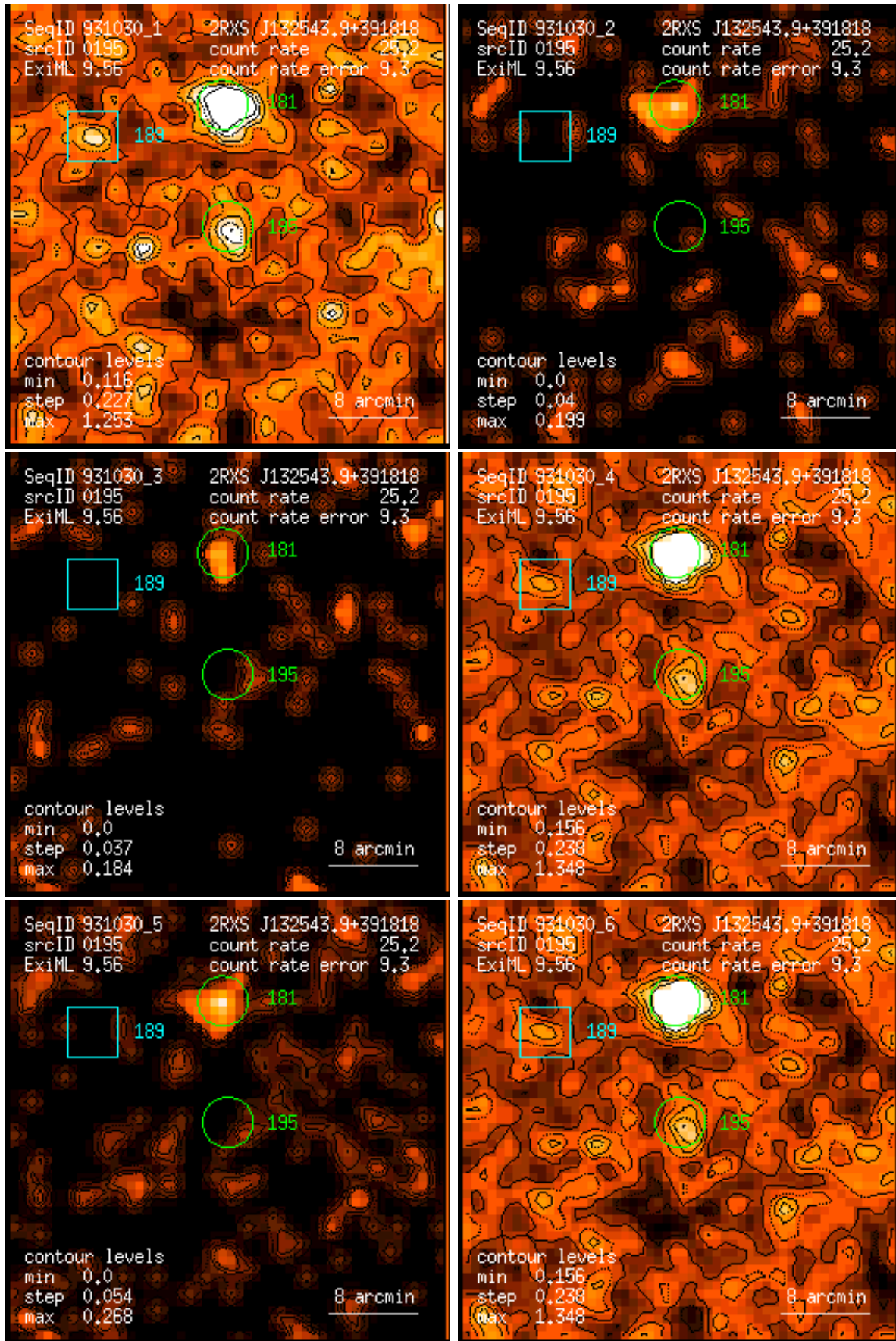
Figure 195: RASS 931030: detection 0195: band rate images, Gaussian filter: (1) PSPC channels 11 – 41, (2) 52 – 90, (3) 91 – 201, (4) 11 – 235, (5) 52 – 201, (6) 11 – 201. Broad band rates in counts/ks. Band rate contour levels in counts/ks/arcmin 2 .
