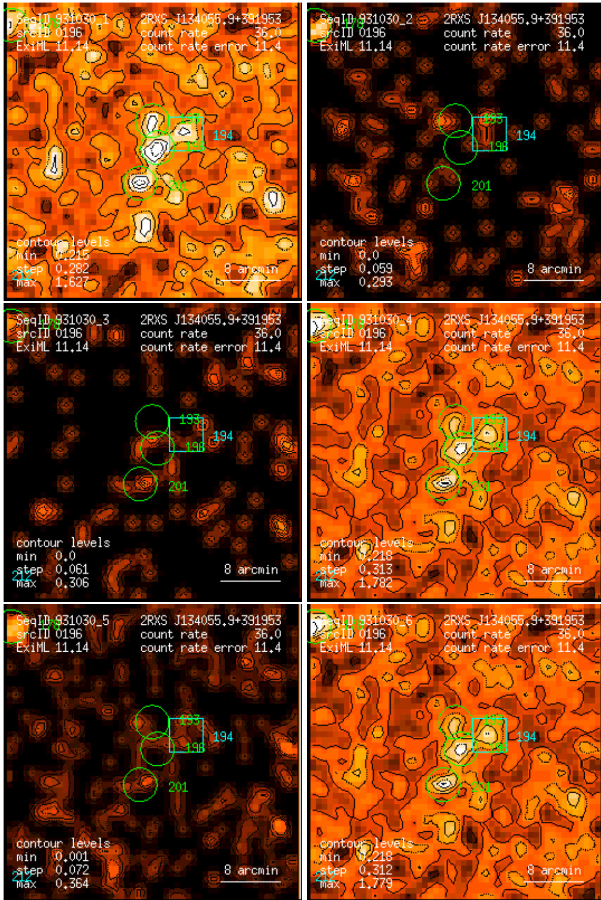
Figure 196: RASS 931030: detection 0196: band rate images, Gaussian filter: (1) PSPC channels 11 – 41, (2) 52 – 90, (3) 91 – 201, (4) 11 – 235, (5) 52 – 201, (6) 11 – 201. Broad band rates in counts/ks. Band rate contour levels in counts/ks/arcmin 2 .
