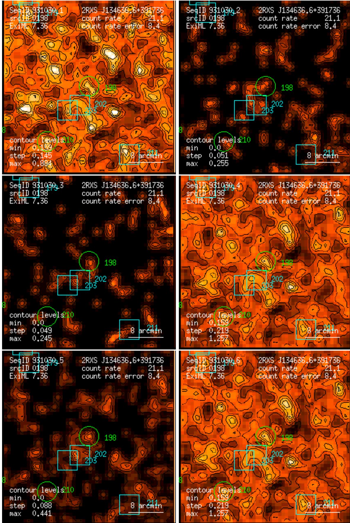
Figure 198: RASS 931030: detection 0198: band rate images, Gaussian filter: (1) PSPC channels 11 – 41, (2) 52 – 90, (3) 91 – 201, (4) 11 – 235, (5) 52 – 201, (6) 11 – 201. Broad band rates in counts/ks. Band rate contour levels in counts/ks/arcmin 2 .
