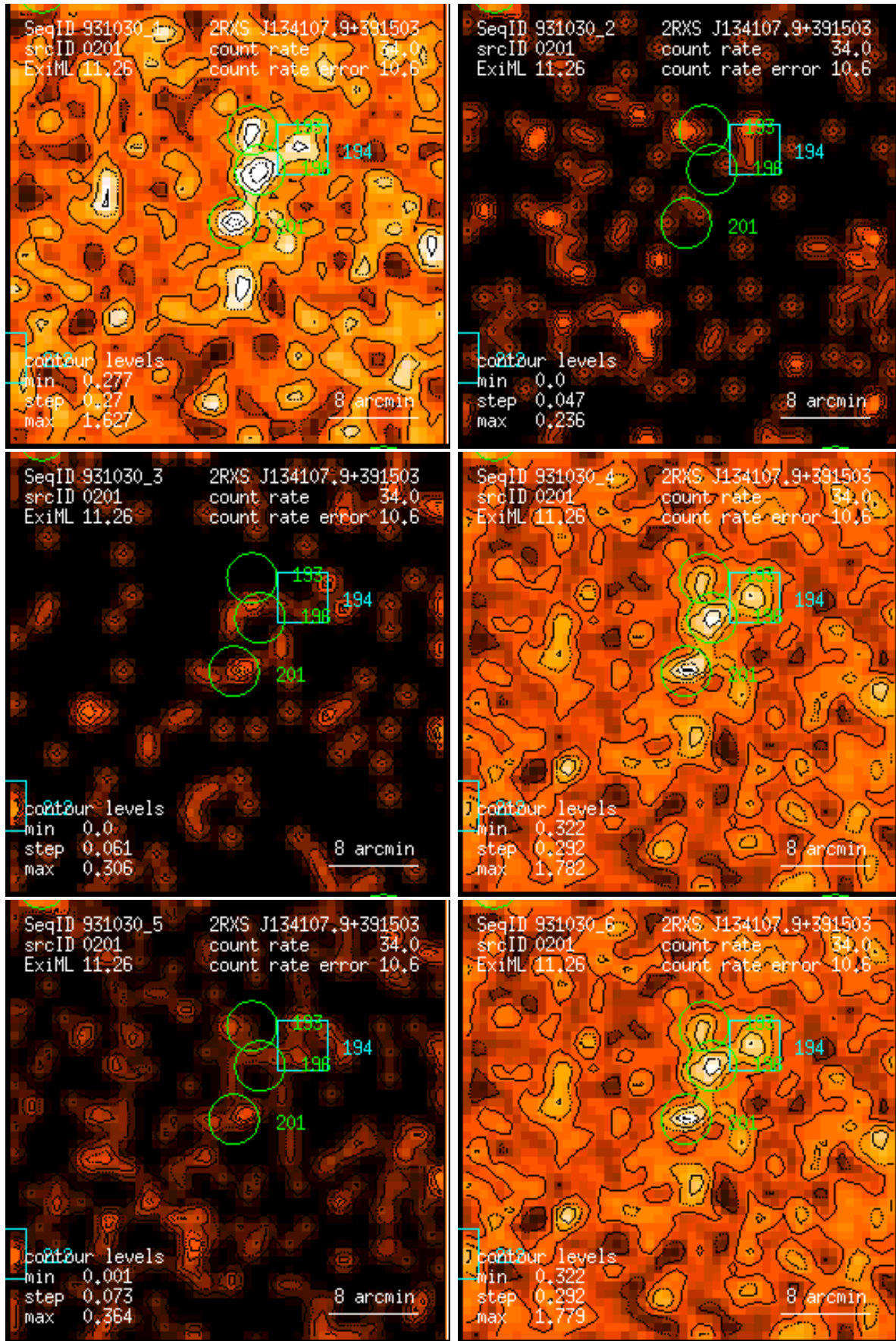
Figure 201: RASS 931030: detection 0201: band rate images, Gaussian filter: (1) PSPC channels 11 – 41, (2) 52 – 90, (3) 91 – 201, (4) 11 – 235, (5) 52 – 201, (6) 11 – 201. Broad band rates in counts/ks. Band rate contour levels in counts/ks/arcmin 2 .
