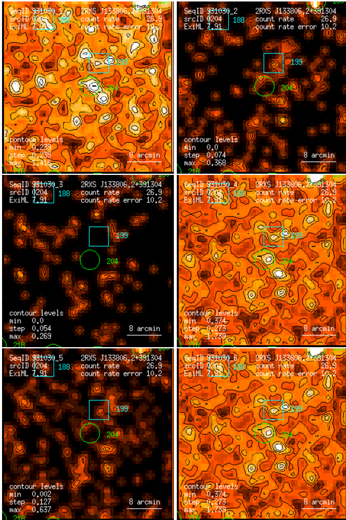
Figure 204: RASS 931030: detection 0204: band rate images, Gaussian filter: (1) PSPC channels 11 – 41, (2) 52 – 90, (3) 91 – 201, (4) 11 – 235, (5) 52 – 201, (6) 11 – 201. Broad band rates in counts/ks. Band rate contour levels in counts/ks/arcmin 2 .
