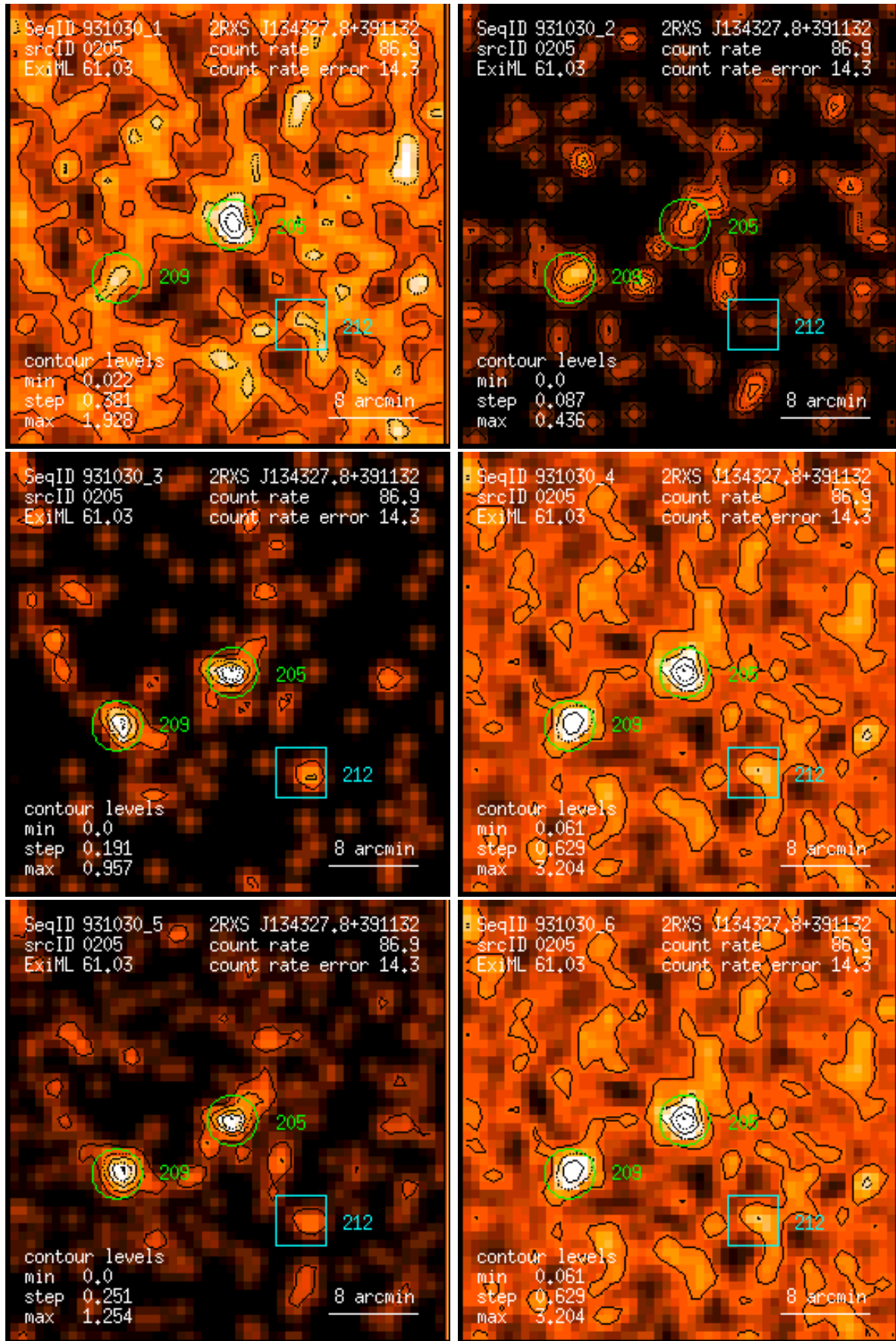
Figure 205: RASS 931030: detection 0205: band rate images, Gaussian filter: (1) PSPC channels 11 – 41, (2) 52 – 90, (3) 91 – 201, (4) 11 – 235, (5) 52 – 201, (6) 11 – 201. Broad band rates in counts/ks. Band rate contour levels in counts/ks/arcmin 2 .
