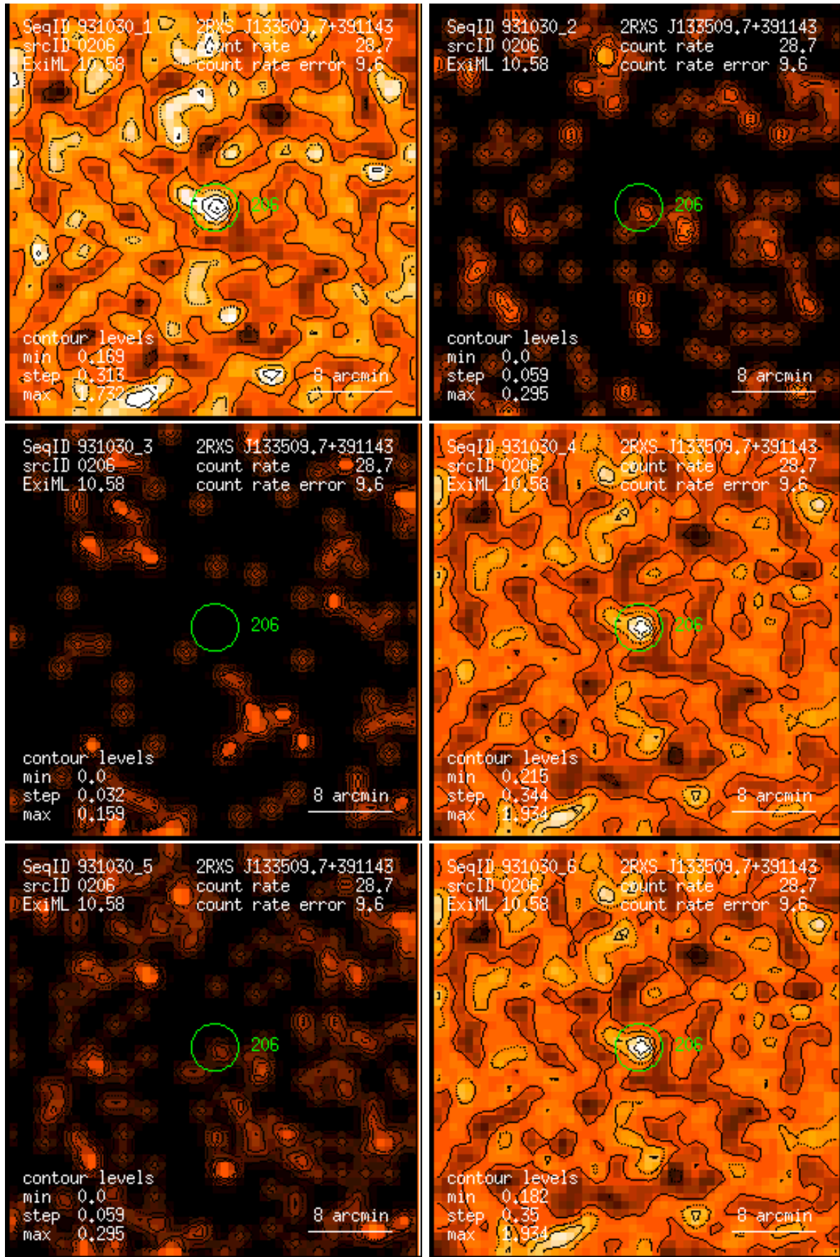
Figure 206: RASS 931030: detection 0206: band rate images, Gaussian filter: (1) PSPC channels 11 – 41, (2) 52 – 90, (3) 91 – 201, (4) 11 – 235, (5) 52 – 201, (6) 11 – 201. Broad band rates in counts/ks. Band rate contour levels in counts/ks/arcmin 2 .
