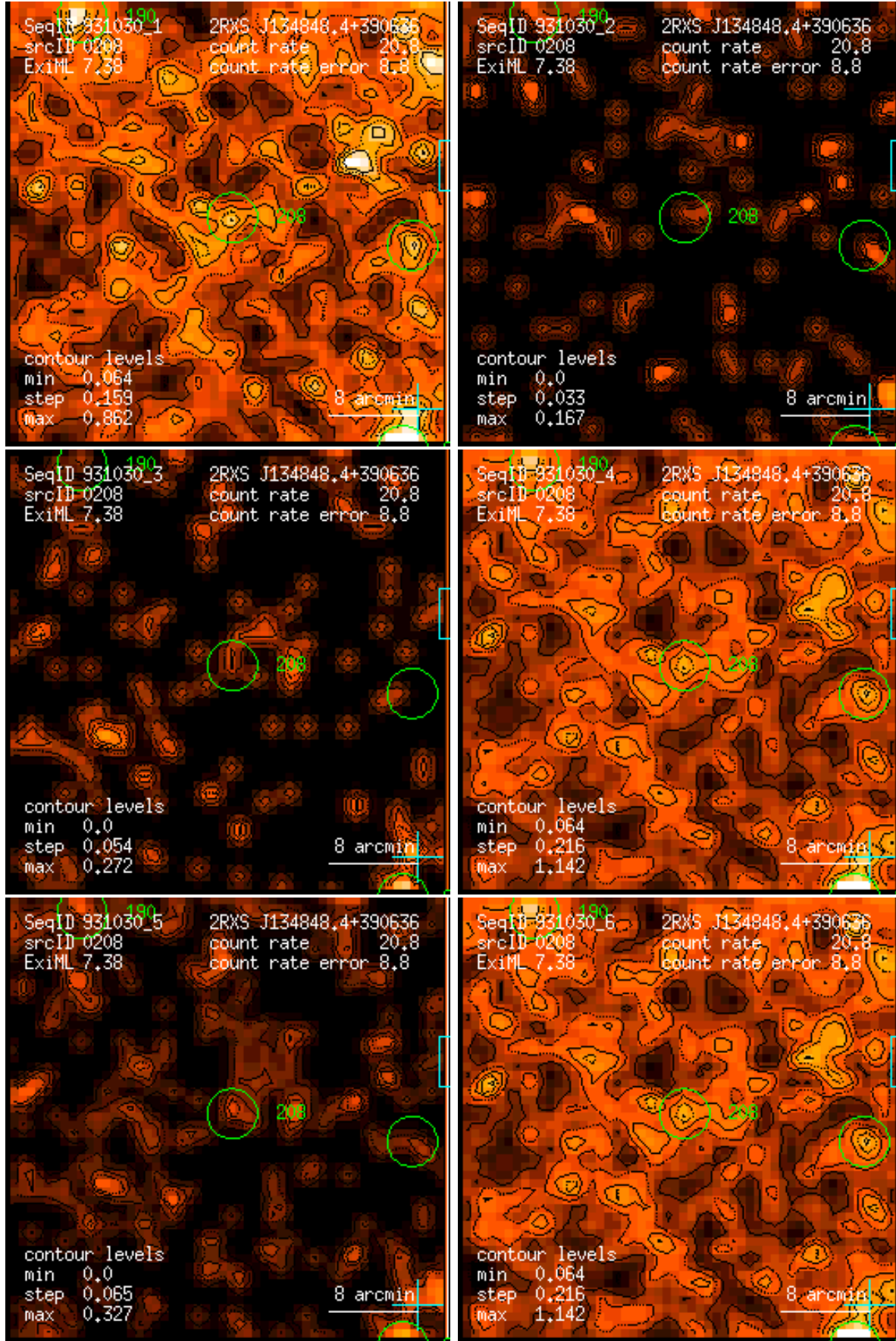
Figure 208: RASS 931030: detection 0208: band rate images, Gaussian filter: (1) PSPC channels 11 – 41, (2) 52 – 90, (3) 91 – 201, (4) 11 – 235, (5) 52 – 201, (6) 11 – 201. Broad band rates in counts/ks. Band rate contour levels in counts/ks/arcmin 2 .
