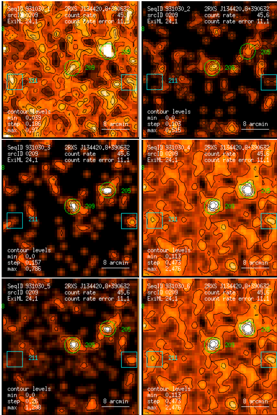
Figure 209: RASS 931030: detection 0209: band rate images, Gaussian filter: (1) PSPC channels 11 – 41, (2) 52 – 90, (3) 91 – 201, (4) 11 – 235, (5) 52 – 201, (6) 11 – 201. Broad band rates in counts/ks. Band rate contour levels in counts/ks/arcmin 2 .
