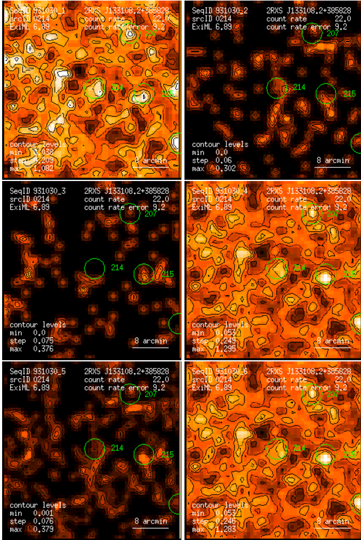
Figure 214: RASS 931030: detection 0214: band rate images, Gaussian filter: (1) PSPC channels 11 – 41, (2) 52 – 90, (3) 91 – 201, (4) 11 – 235, (5) 52 – 201, (6) 11 – 201. Broad band rates in counts/ks. Band rate contour levels in counts/ks/arcmin 2 .
