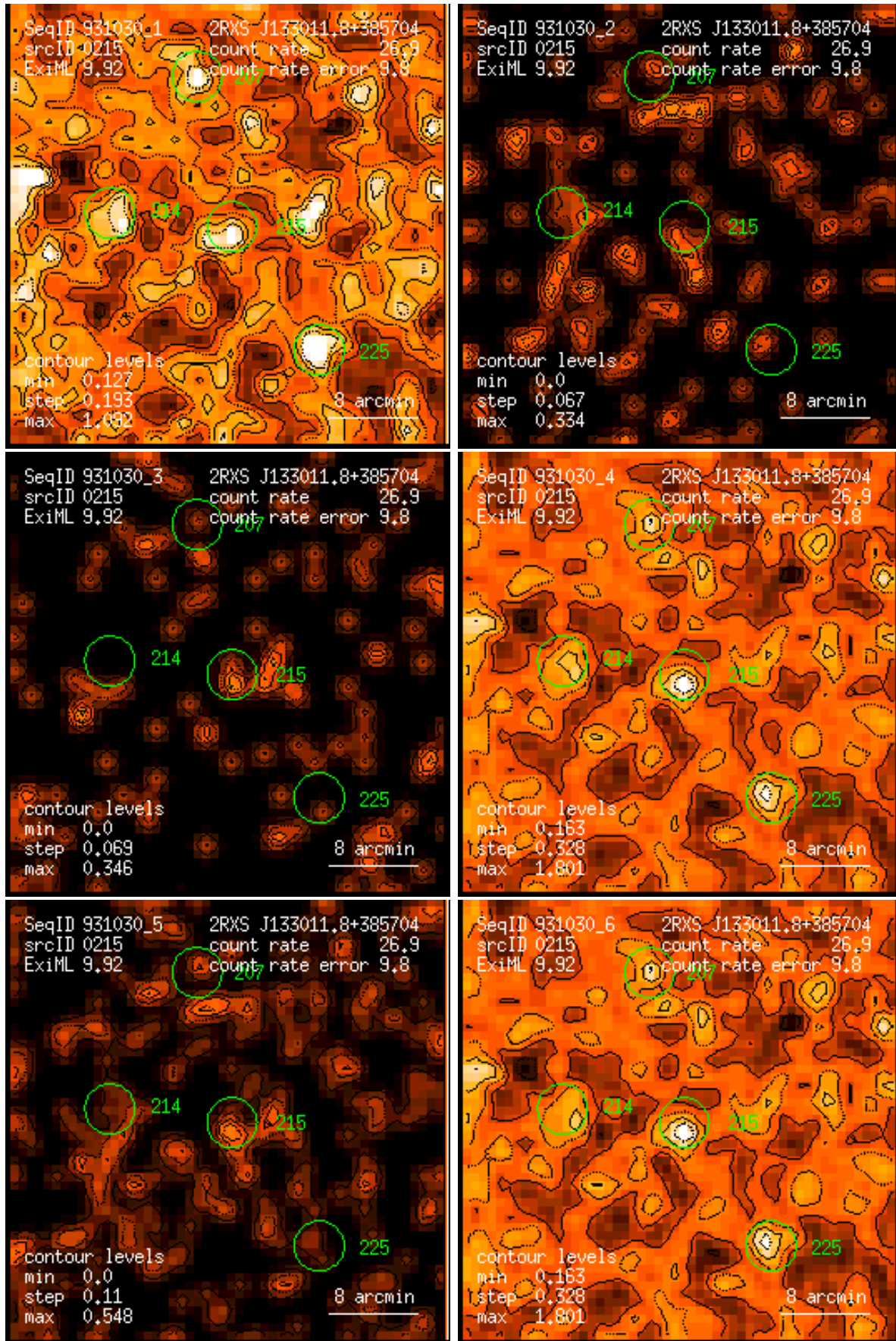
Figure 215: RASS 931030: detection 0215: band rate images, Gaussian filter: (1) PSPC channels 11 – 41, (2) 52 – 90, (3) 91 – 201, (4) 11 – 235, (5) 52 – 201, (6) 11 – 201. Broad band rates in counts/ks. Band rate contour levels in counts/ks/arcmin 2 .
