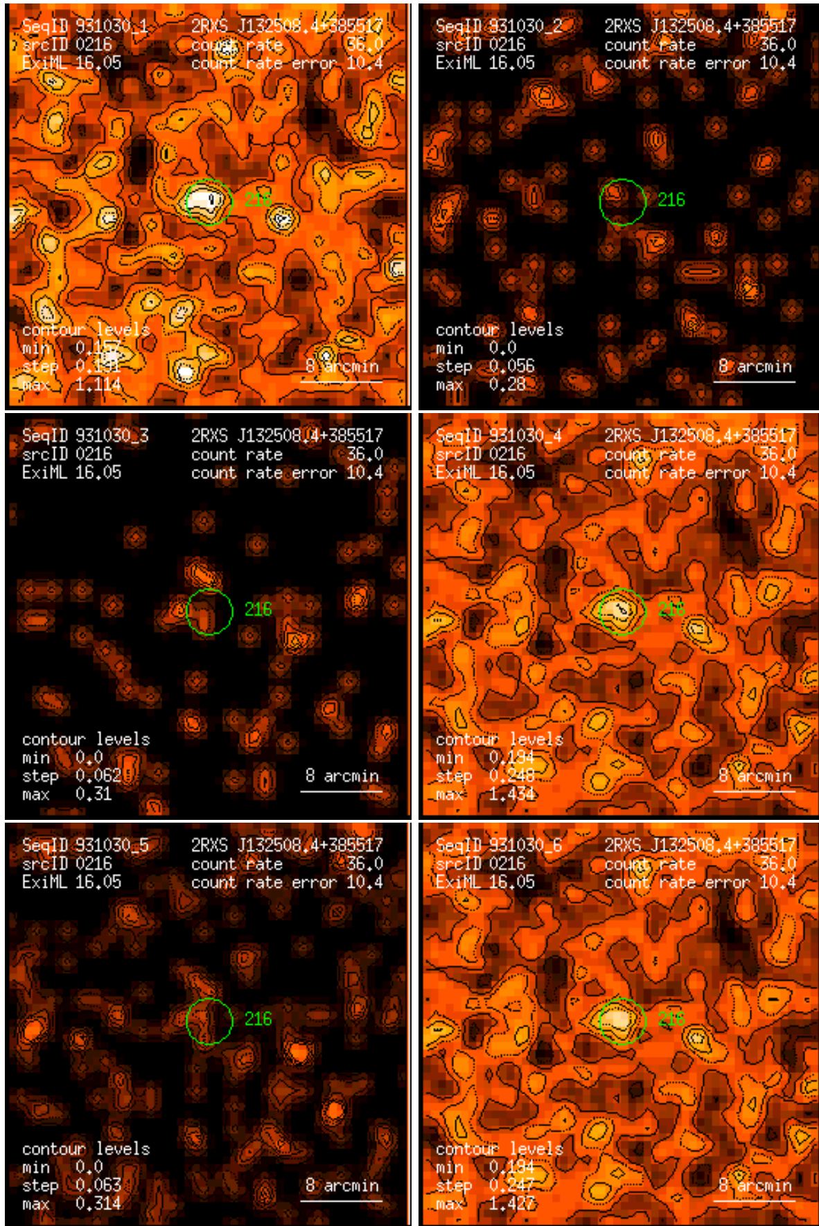
Figure 216: RASS 931030: detection 0216: band rate images, Gaussian filter: (1) PSPC channels 11 – 41, (2) 52 – 90, (3) 91 – 201, (4) 11 – 235, (5) 52 – 201, (6) 11 – 201. Broad band rates in counts/ks. Band rate contour levels in counts/ks/arcmin 2 .
