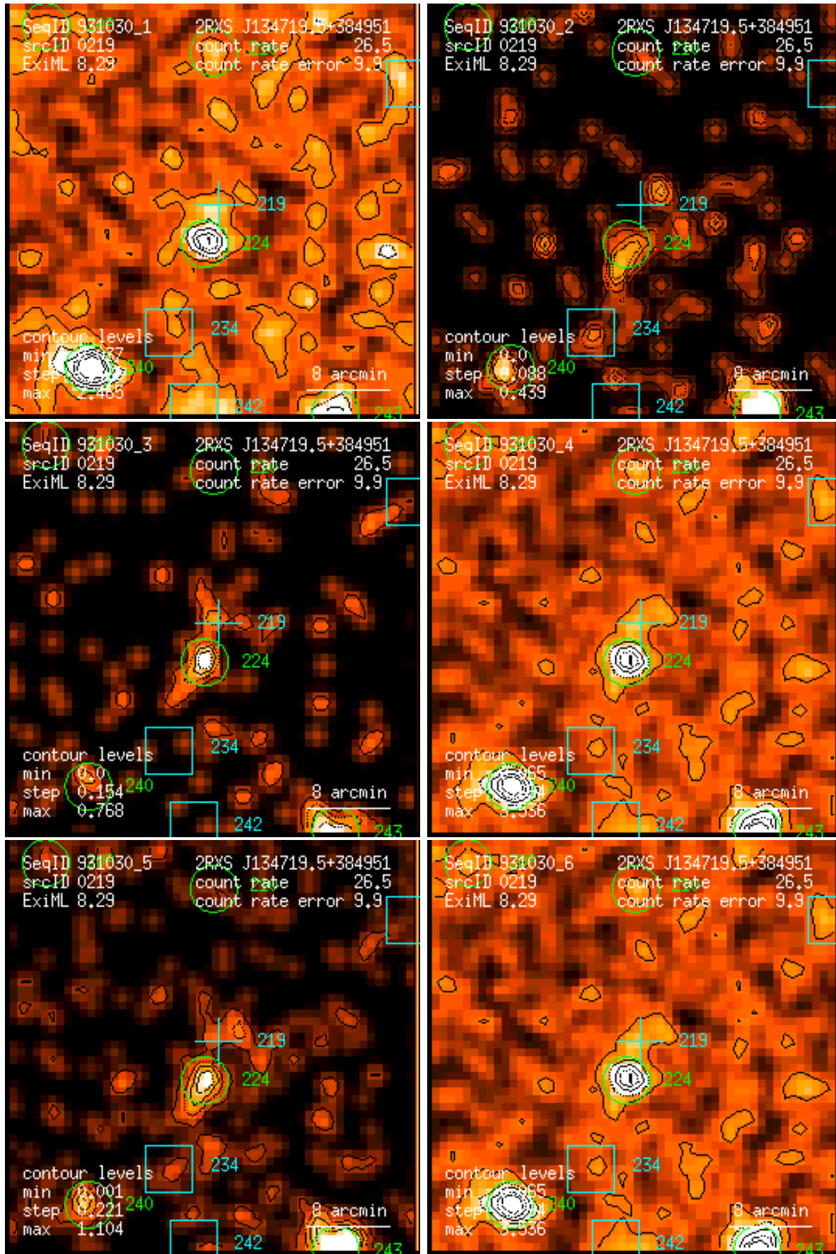
Figure 219: RASS 931030: detection 0219: band rate images, Gaussian filter: (1) PSPC channels 11 – 41, (2) 52 – 90, (3) 91 – 201, (4) 11 – 235, (5) 52 – 201, (6) 11 – 201. Broad band rates in counts/ks. Band rate contour levels in counts/ks/arcmin 2 .
