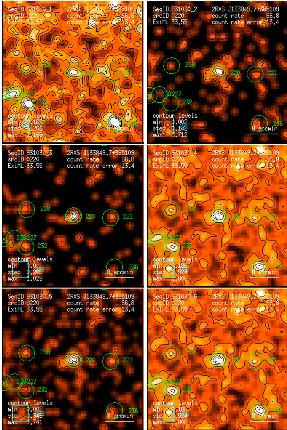
Figure 220: RASS 931030: detection 0220: band rate images, Gaussian filter: (1) PSPC channels 11 – 41, (2) 52 – 90, (3) 91 – 201, (4) 11 – 235, (5) 52 – 201, (6) 11 – 201. Broad band rates in counts/ks. Band rate contour levels in counts/ks/arcmin 2 .
