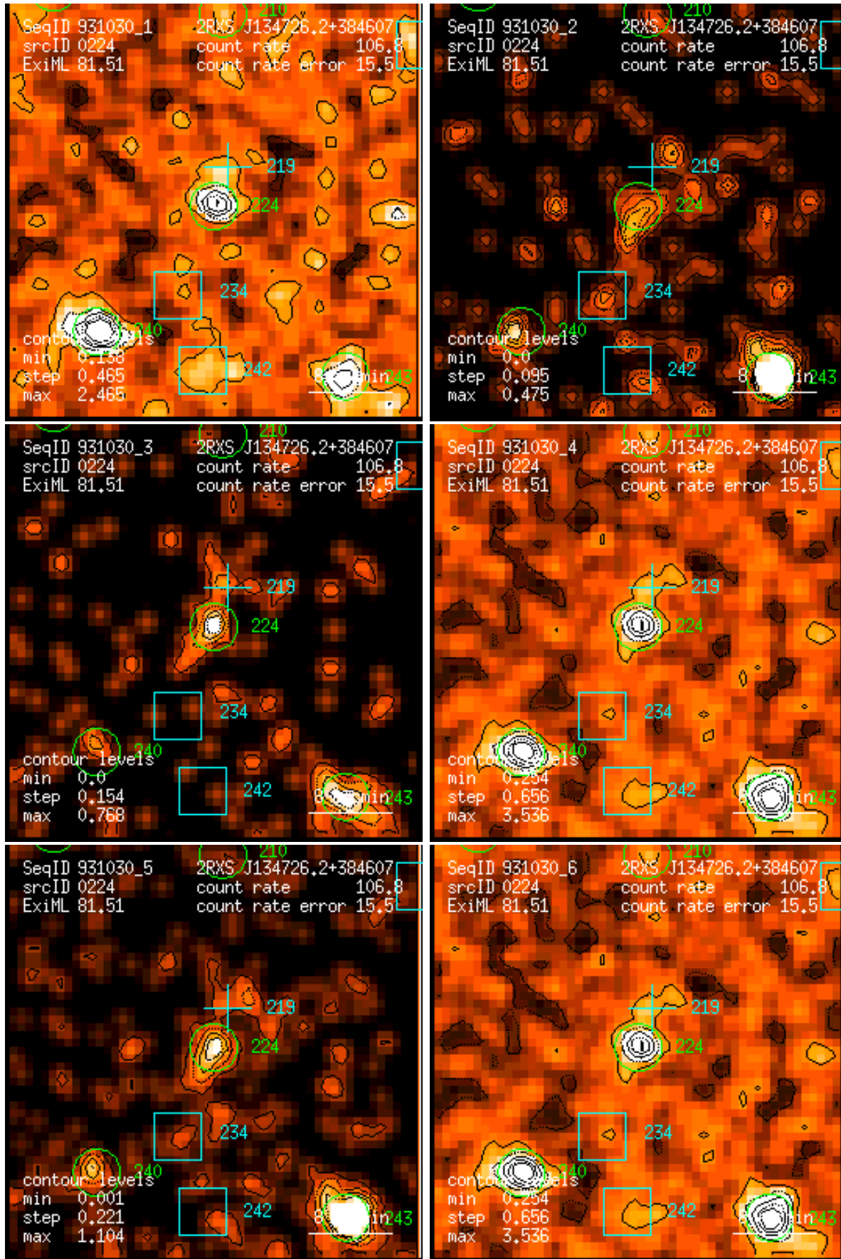
Figure 224: RASS 931030: detection 0224: band rate images, Gaussian filter: (1) PSPC channels 11 – 41, (2) 52 – 90, (3) 91 – 201, (4) 11 – 235, (5) 52 – 201, (6) 11 – 201. Broad band rates in counts/ks. Band rate contour levels in counts/ks/arcmin 2 .
