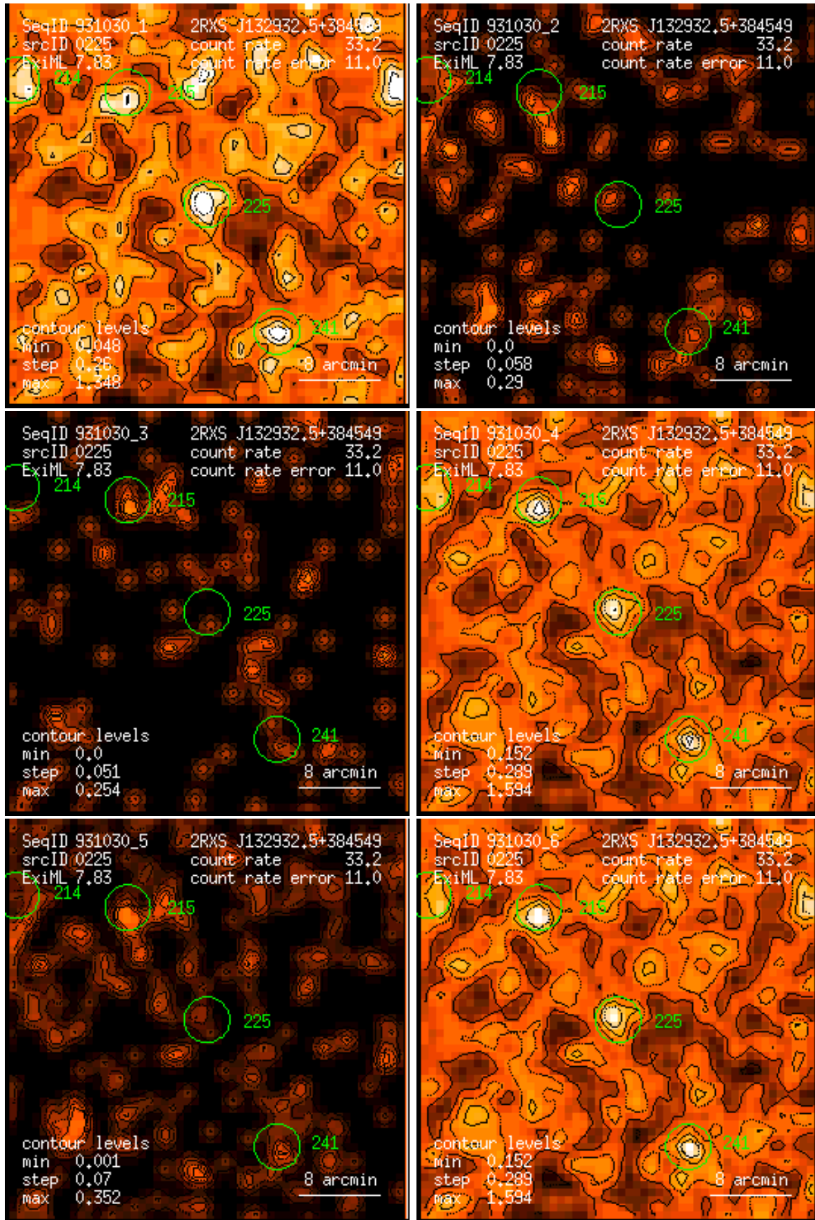
Figure 225: RASS 931030: detection 0225: band rate images, Gaussian filter: (1) PSPC channels 11 – 41, (2) 52 – 90, (3) 91 – 201, (4) 11 – 235, (5) 52 – 201, (6) 11 – 201. Broad band rates in counts/ks. Band rate contour levels in counts/ks/arcmin 2 .
