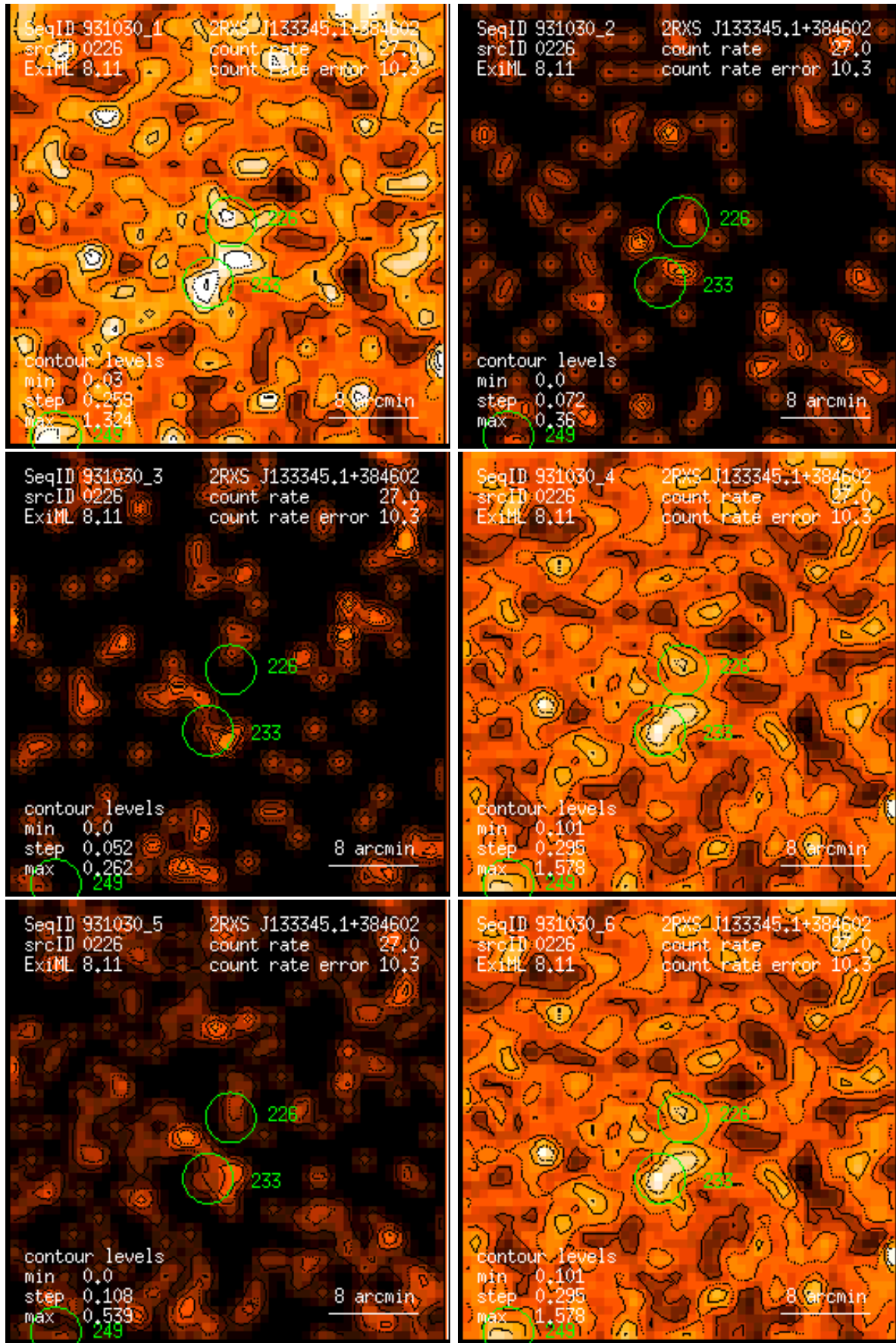
Figure 226: RASS 931030: detection 0226: band rate images, Gaussian filter: (1) PSPC channels 11 – 41, (2) 52 – 90, (3) 91 – 201, (4) 11 – 235, (5) 52 – 201, (6) 11 – 201. Broad band rates in counts/ks. Band rate contour levels in counts/ks/arcmin 2 .
