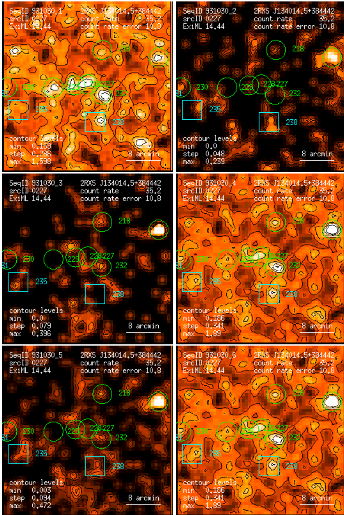
Figure 227: RASS 931030: detection 0227: band rate images, Gaussian filter: (1) PSPC channels 11 – 41, (2) 52 – 90, (3) 91 – 201, (4) 11 – 235, (5) 52 – 201, (6) 11 – 201. Broad band rates in counts/ks. Band rate contour levels in counts/ks/arcmin 2 .
