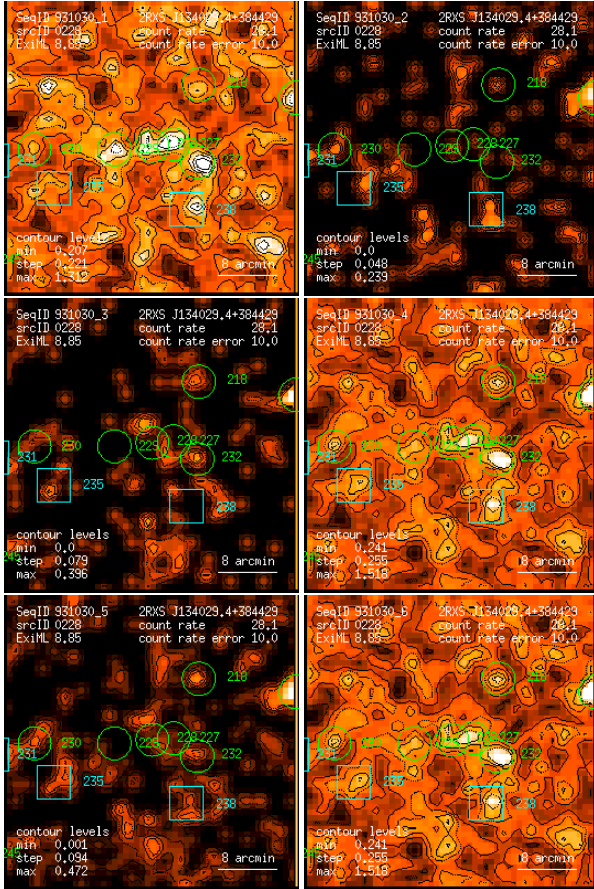
Figure 228: RASS 931030: detection 0228: band rate images, Gaussian filter: (1) PSPC channels 11 – 41, (2) 52 – 90, (3) 91 – 201, (4) 11 – 235, (5) 52 – 201, (6) 11 – 201. Broad band rates in counts/ks. Band rate contour levels in counts/ks/arcmin 2 .
