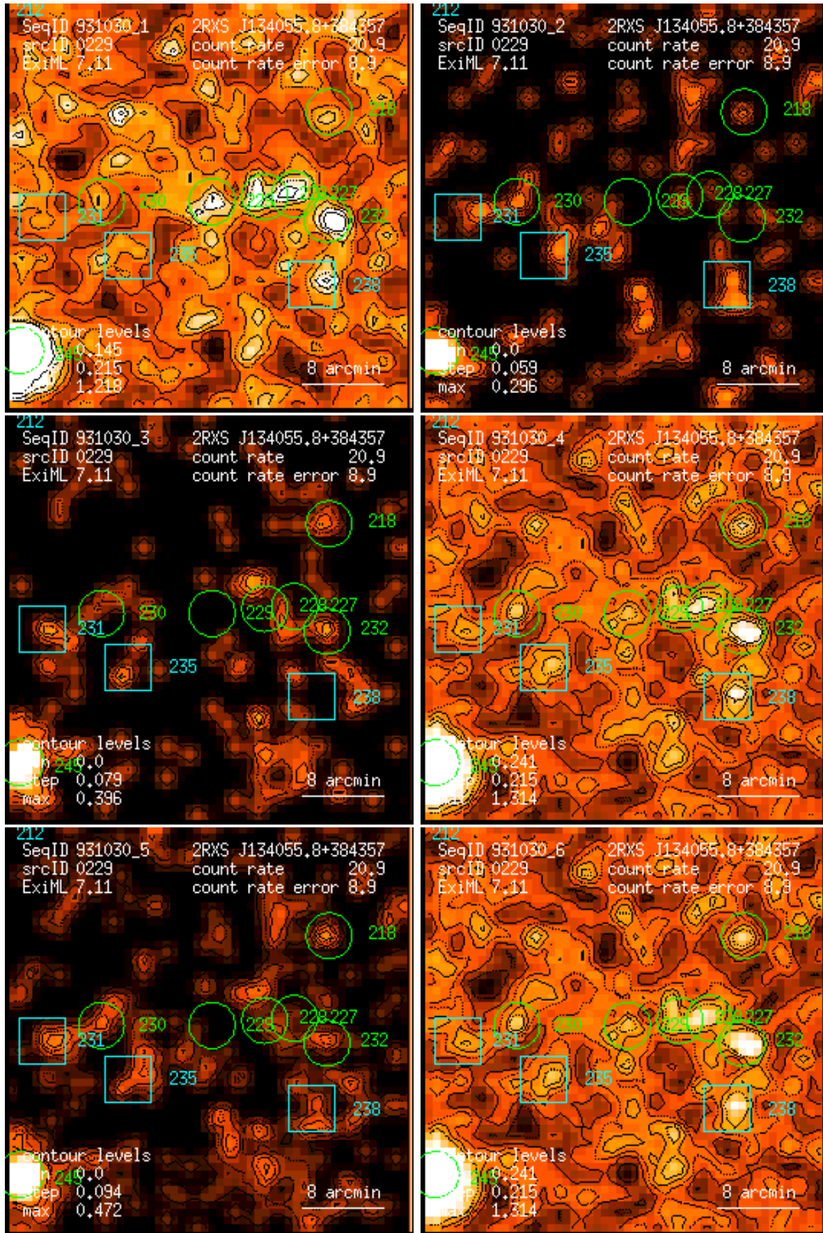
Figure 229: RASS 931030: detection 0229: band rate images, Gaussian filter: (1) PSPC channels 11 – 41, (2) 52 – 90, (3) 91 – 201, (4) 11 – 235, (5) 52 – 201, (6) 11 – 201. Broad band rates in counts/ks. Band rate contour levels in counts/ks/arcmin 2 .
