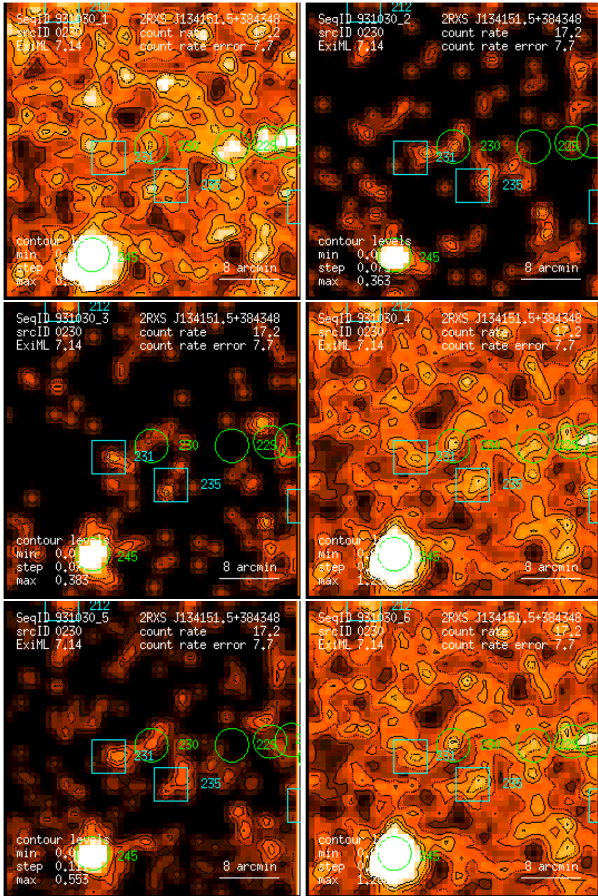
Figure 230: RASS 931030: detection 0230: band rate images, Gaussian filter: (1) PSPC channels 11 – 41, (2) 52 – 90, (3) 91 – 201, (4) 11 – 235, (5) 52 – 201, (6) 11 – 201. Broad band rates in counts/ks. Band rate contour levels in counts/ks/arcmin 2 .
