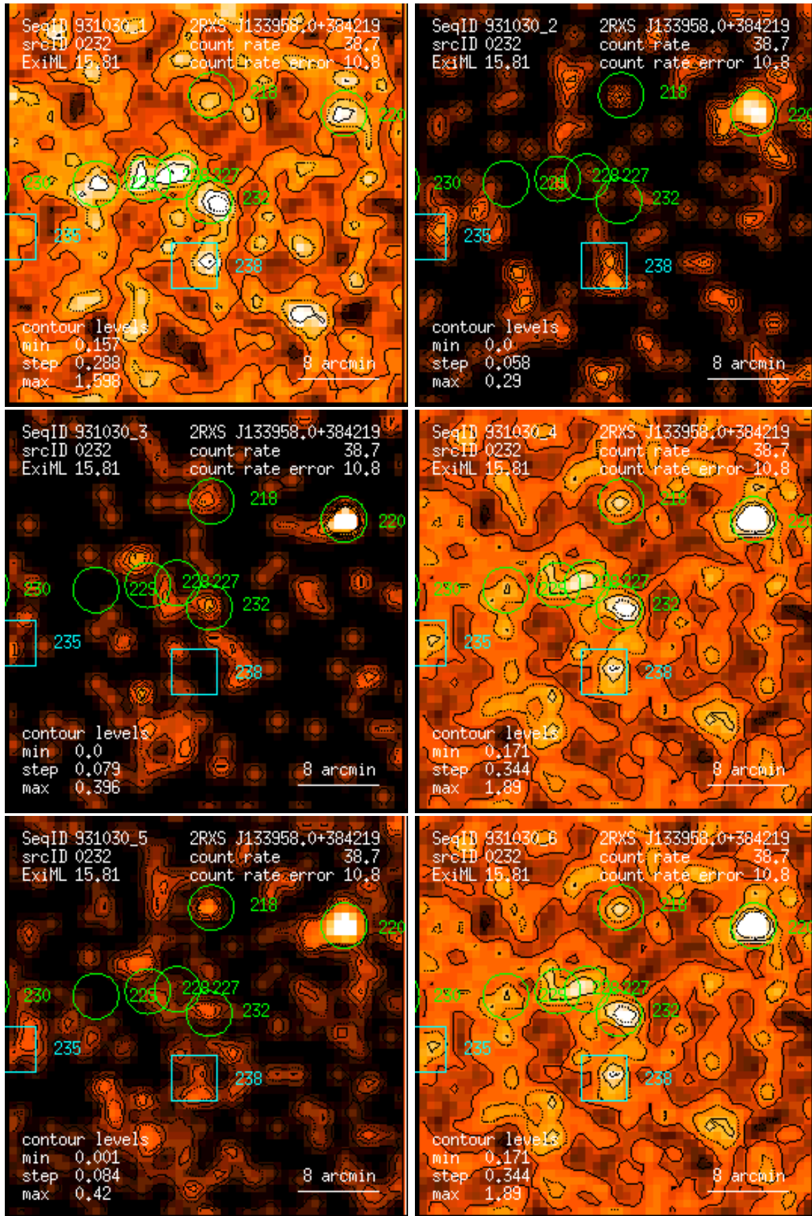
Figure 232: RASS 931030: detection 0232: band rate images, Gaussian filter: (1) PSPC channels 11 – 41, (2) 52 – 90, (3) 91 – 201, (4) 11 – 235, (5) 52 – 201, (6) 11 – 201. Broad band rates in counts/ks. Band rate contour levels in counts/ks/arcmin 2 .
