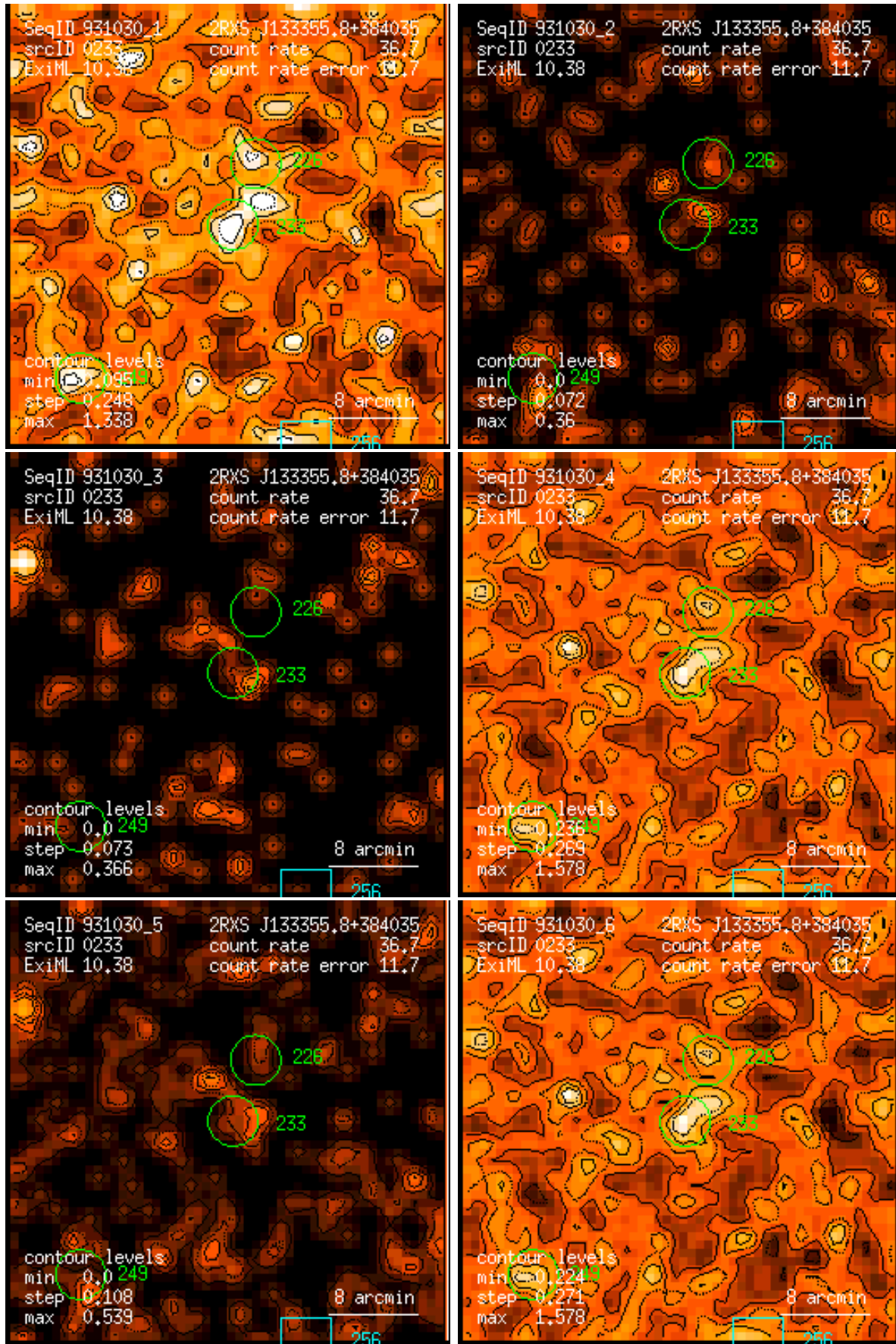
Figure 233: RASS 931030: detection 0233: band rate images, Gaussian filter: (1) PSPC channels 11 – 41, (2) 52 – 90, (3) 91 – 201, (4) 11 – 235, (5) 52 – 201, (6) 11 – 201. Broad band rates in counts/ks. Band rate contour levels in counts/ks/arcmin 2 .
